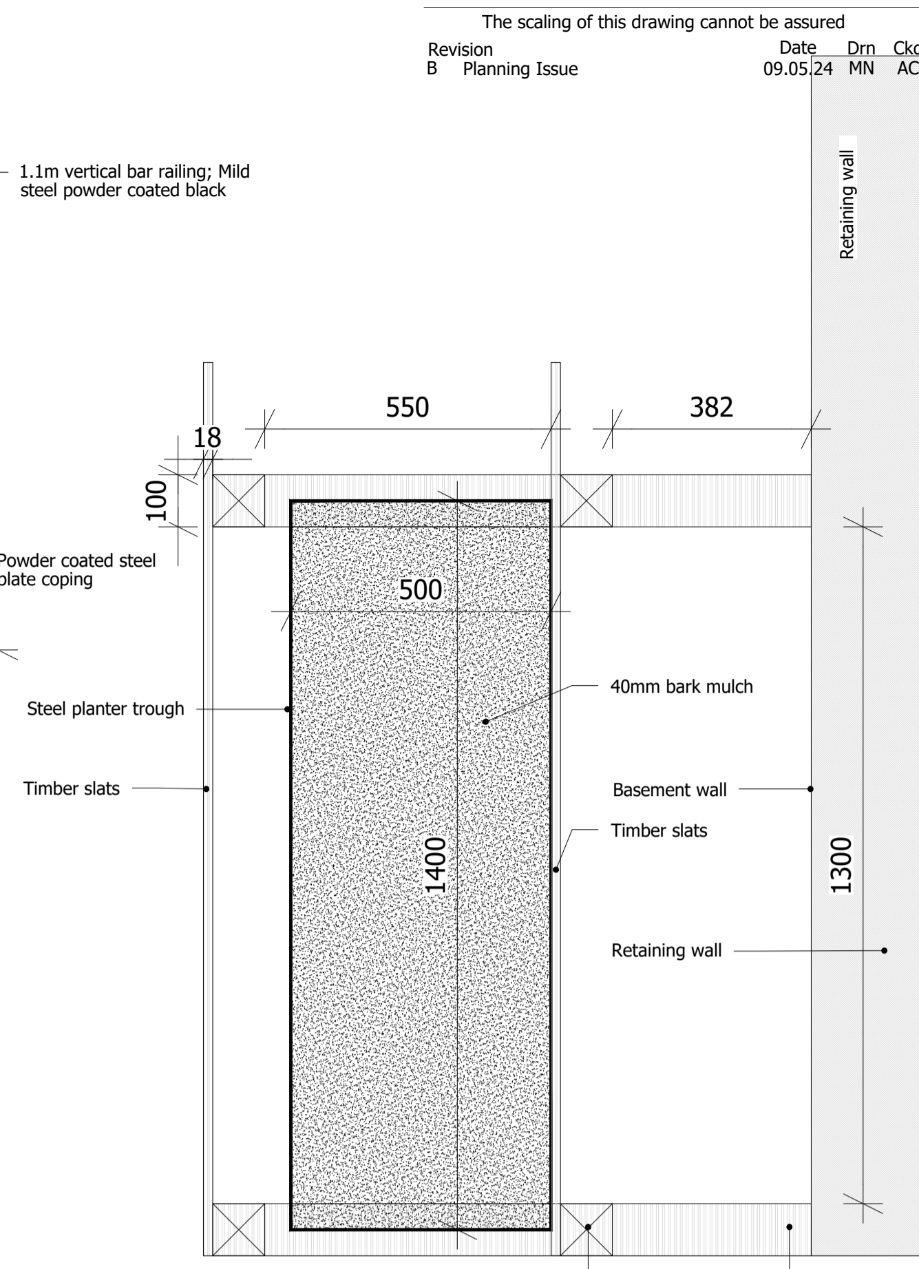
12 Planter Plan View SCALE 1:10@A1
