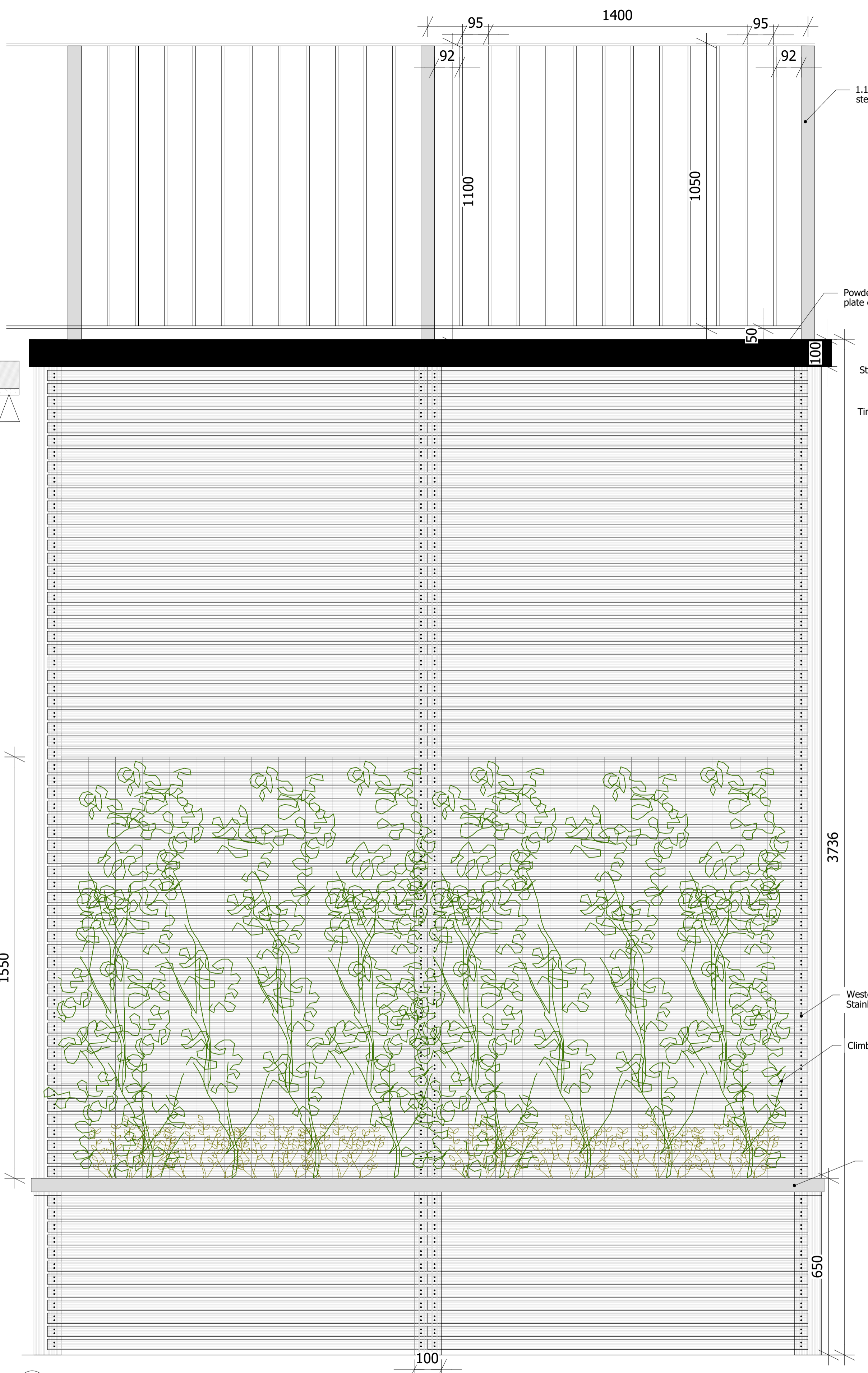
11 Wall Elevation SCALE 1:10@A1
