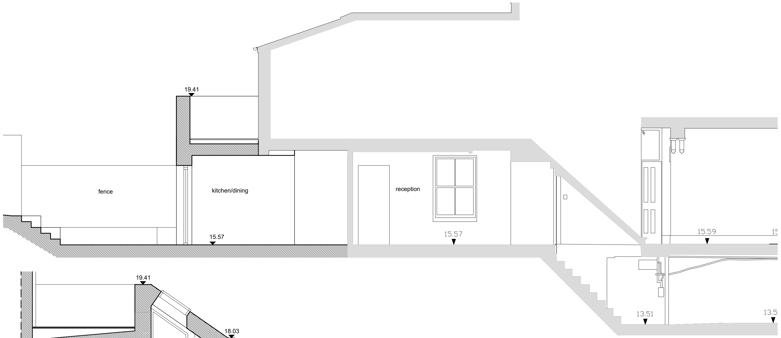
Section AA
