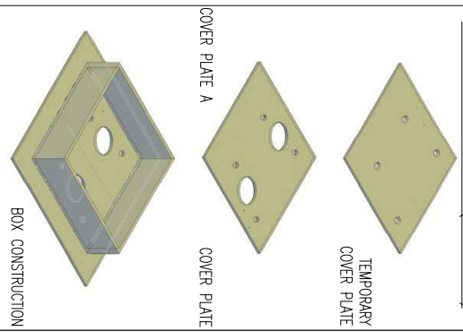
DOCKING POINT BOX CONSTRUCTION DETAILS - (SCALE 1:10)
