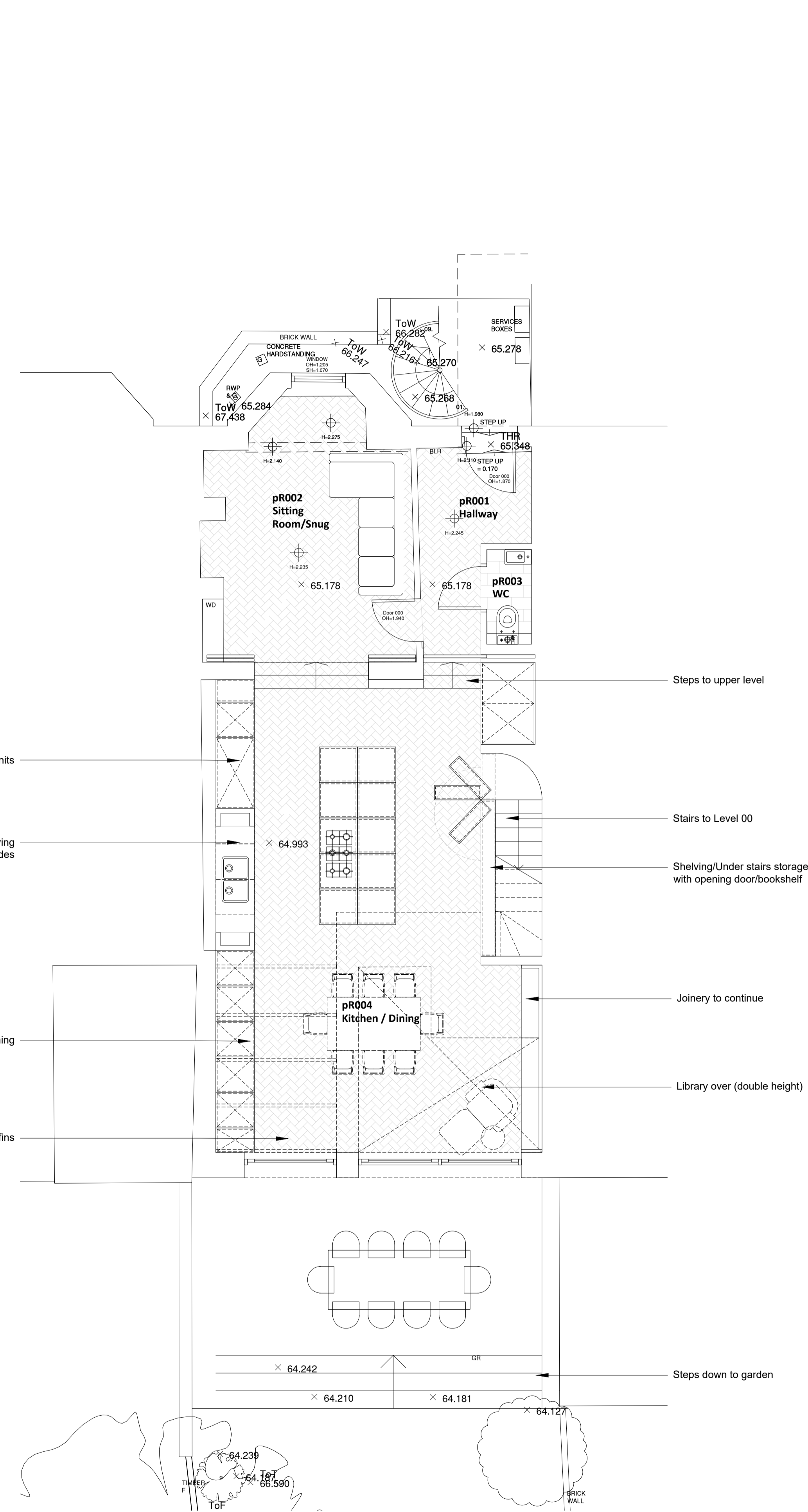
(00) ① PROPOSED PLAN LEVEL (00) 0 0.5 1 2 3 4 5m 1:50
