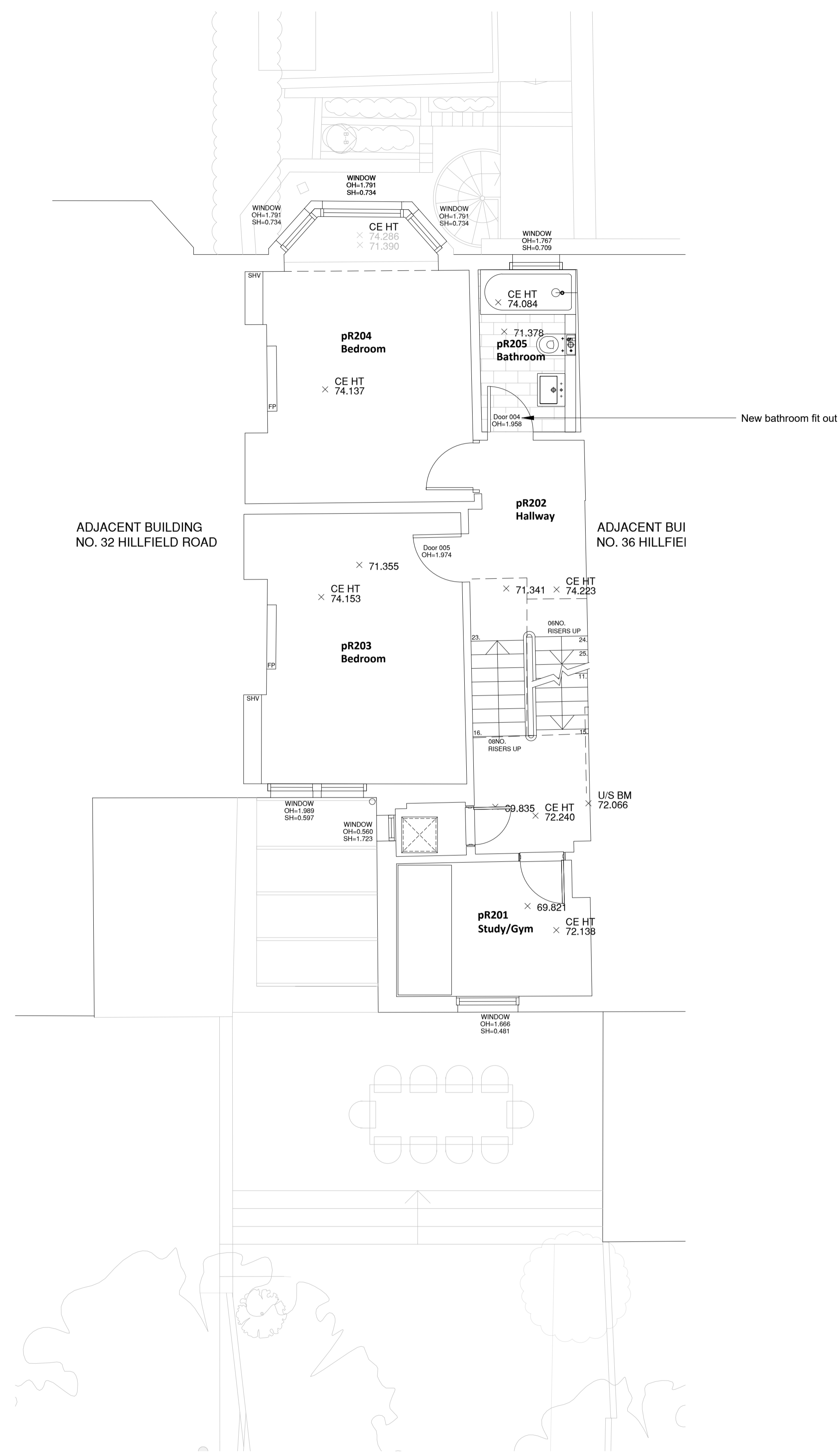
(02) PROPOSED PLAN LEVEL (02) 0 0.5 1 2 3 4 5m 1:50
