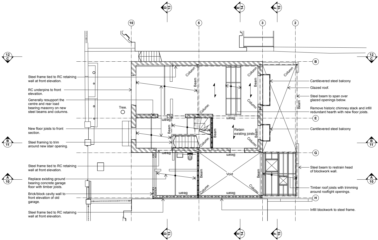
02_GROUND FLOOR
