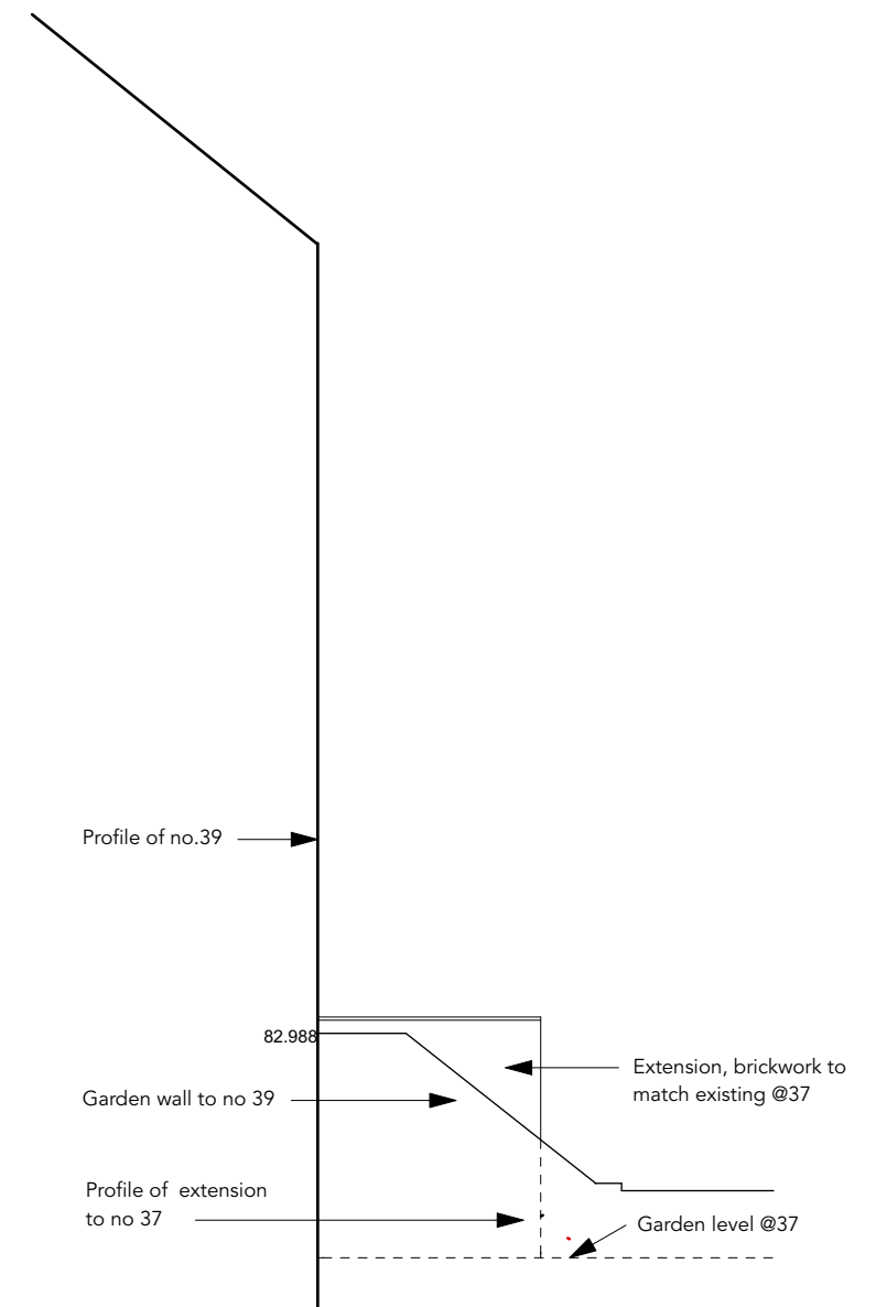
2 side elevation from no 39
