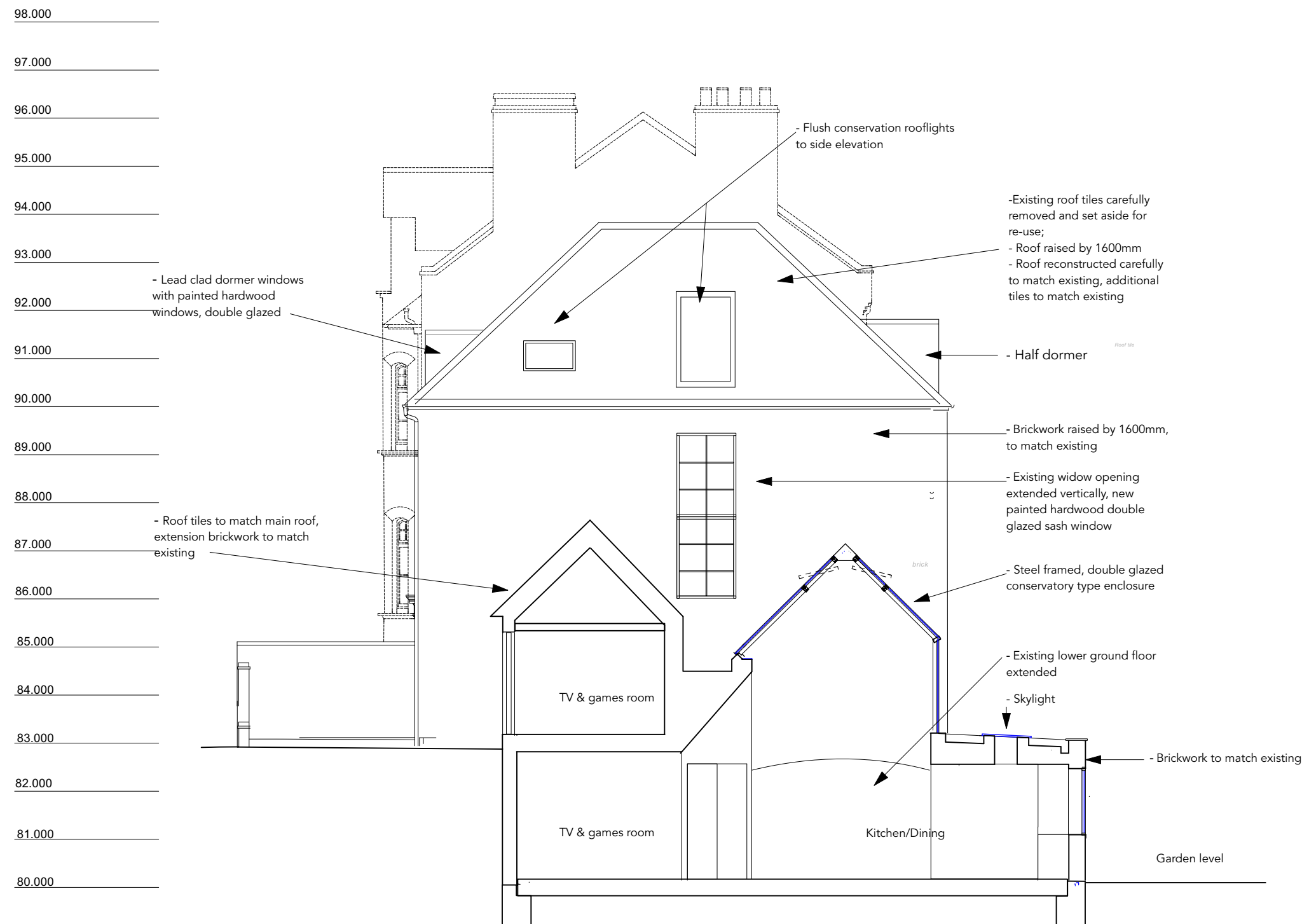
1 side elevation/section through side extension
