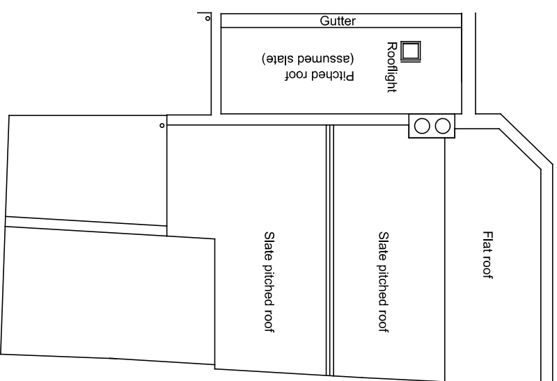
ROOF PLAN
