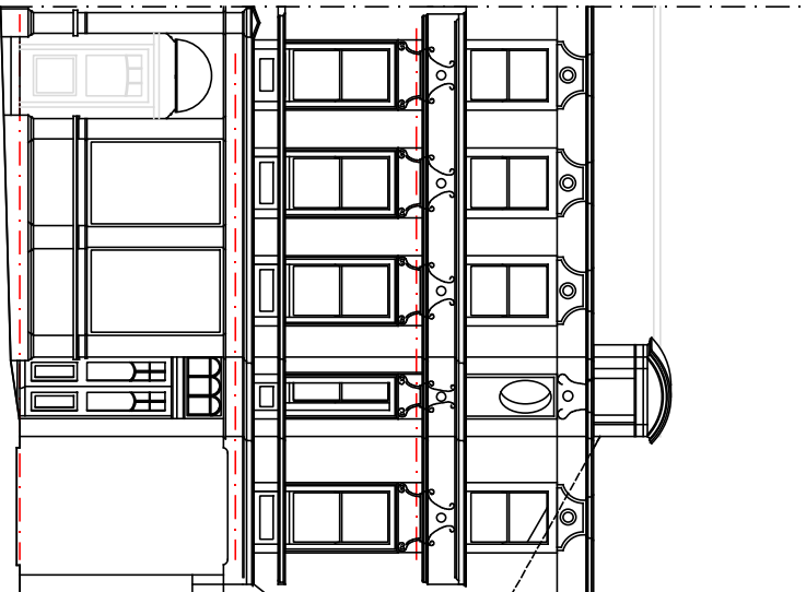
NORTH ELEVATION
