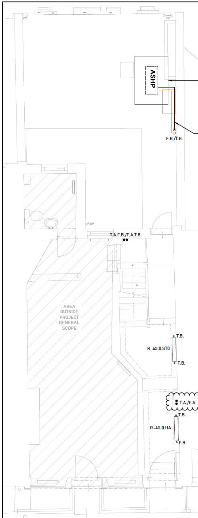
Figure 2: ASHP location
