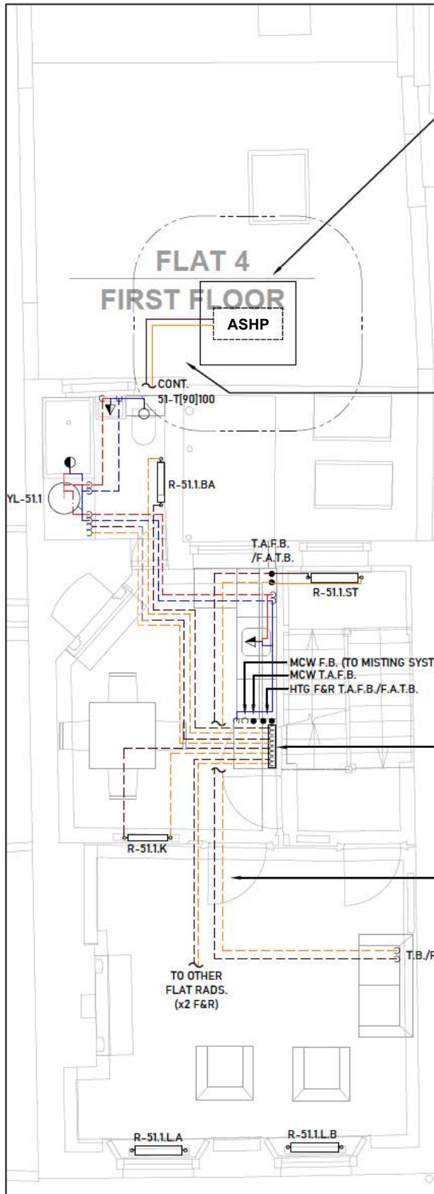
Figure 2: ASHP location
