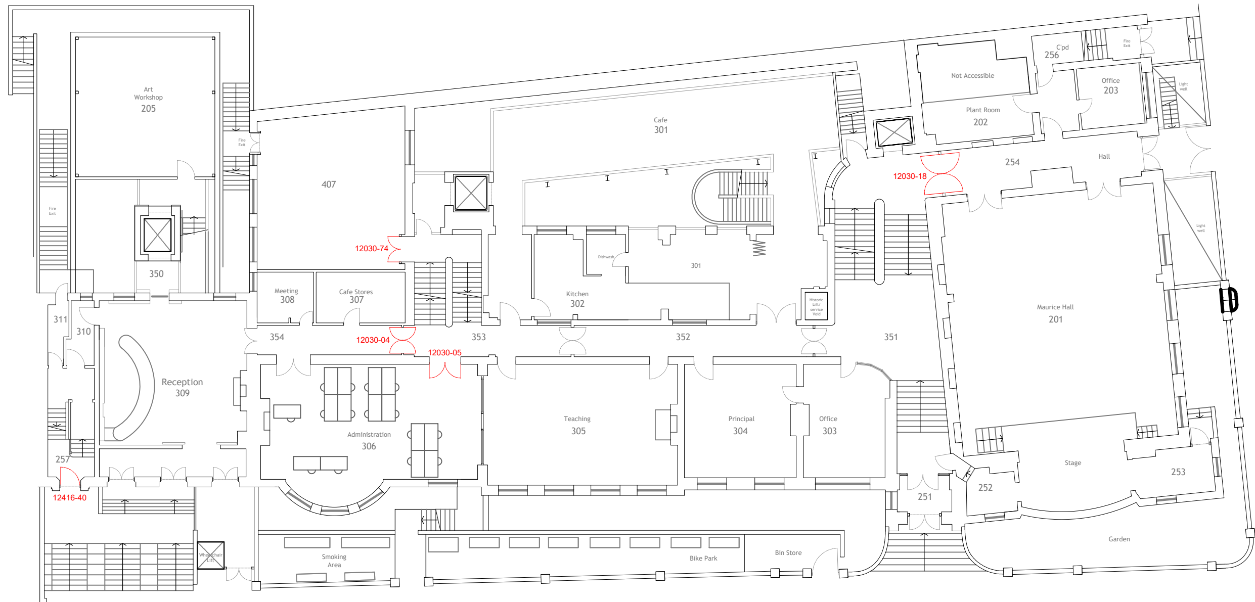
LEVEL 3 FLOOR PLAN Scale 1:200 @ A3
