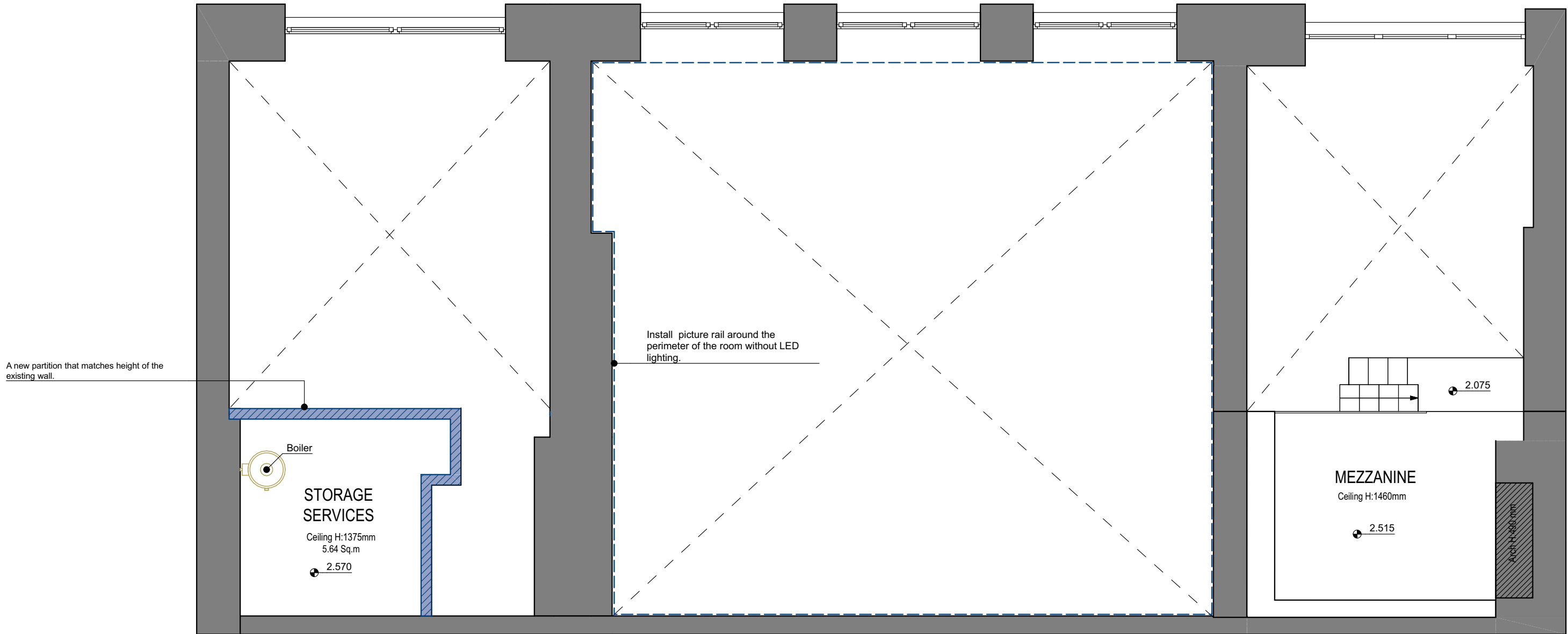
9 PROPOSED STORAGE PLAN SCALE 1:50@A3
