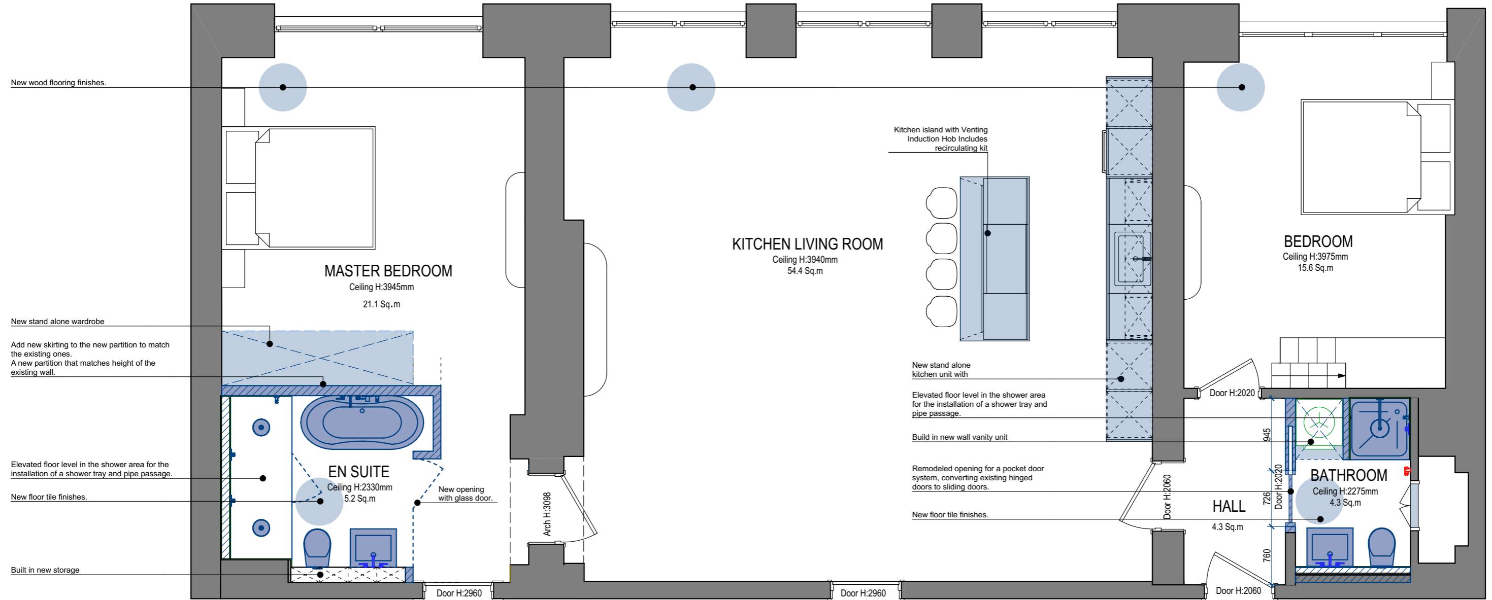
6 PROPOSED PLAN SCALE 1:50@A3
