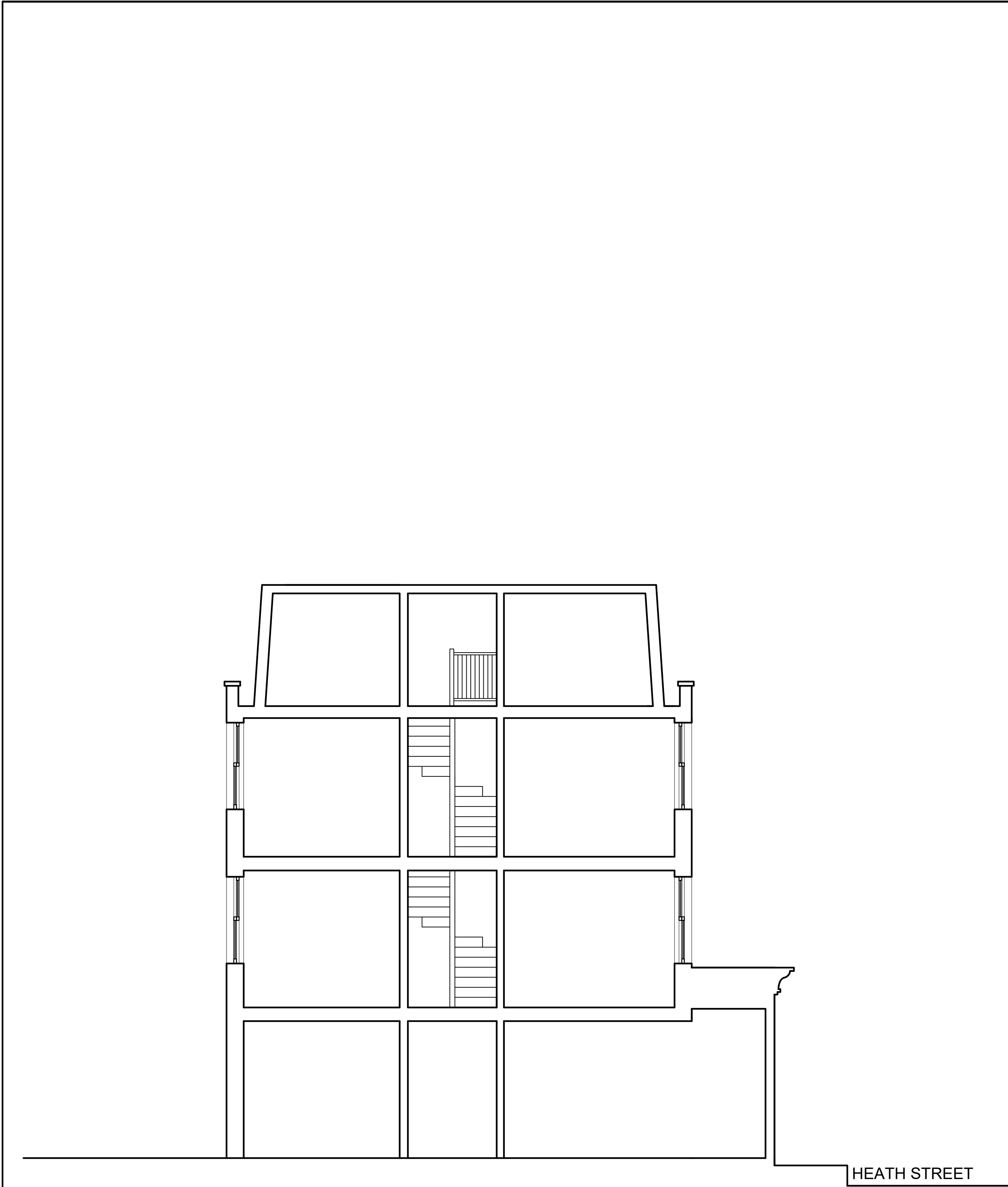
EXISTING SECTION
