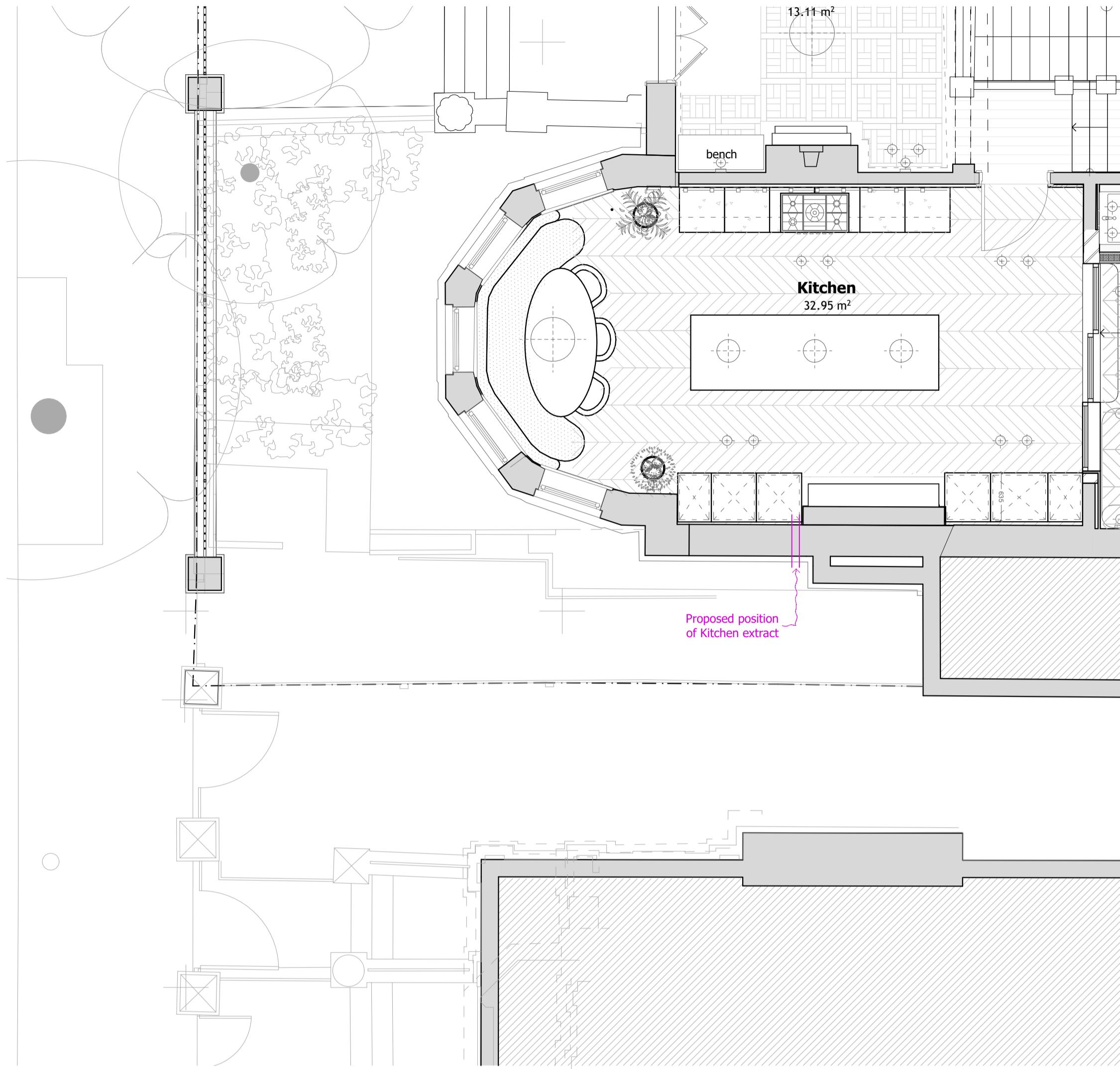
1 Proposed position of Kitchen Extract - Plan
