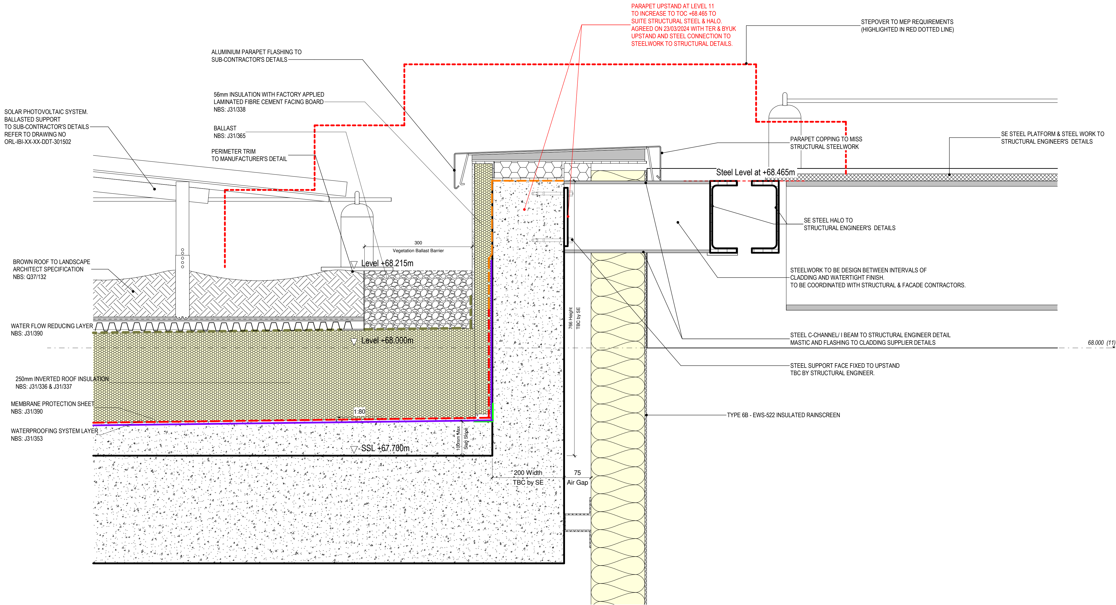
1 Roof Detail, Eleventh Floor, Parapet to Halo Decking 1:5
