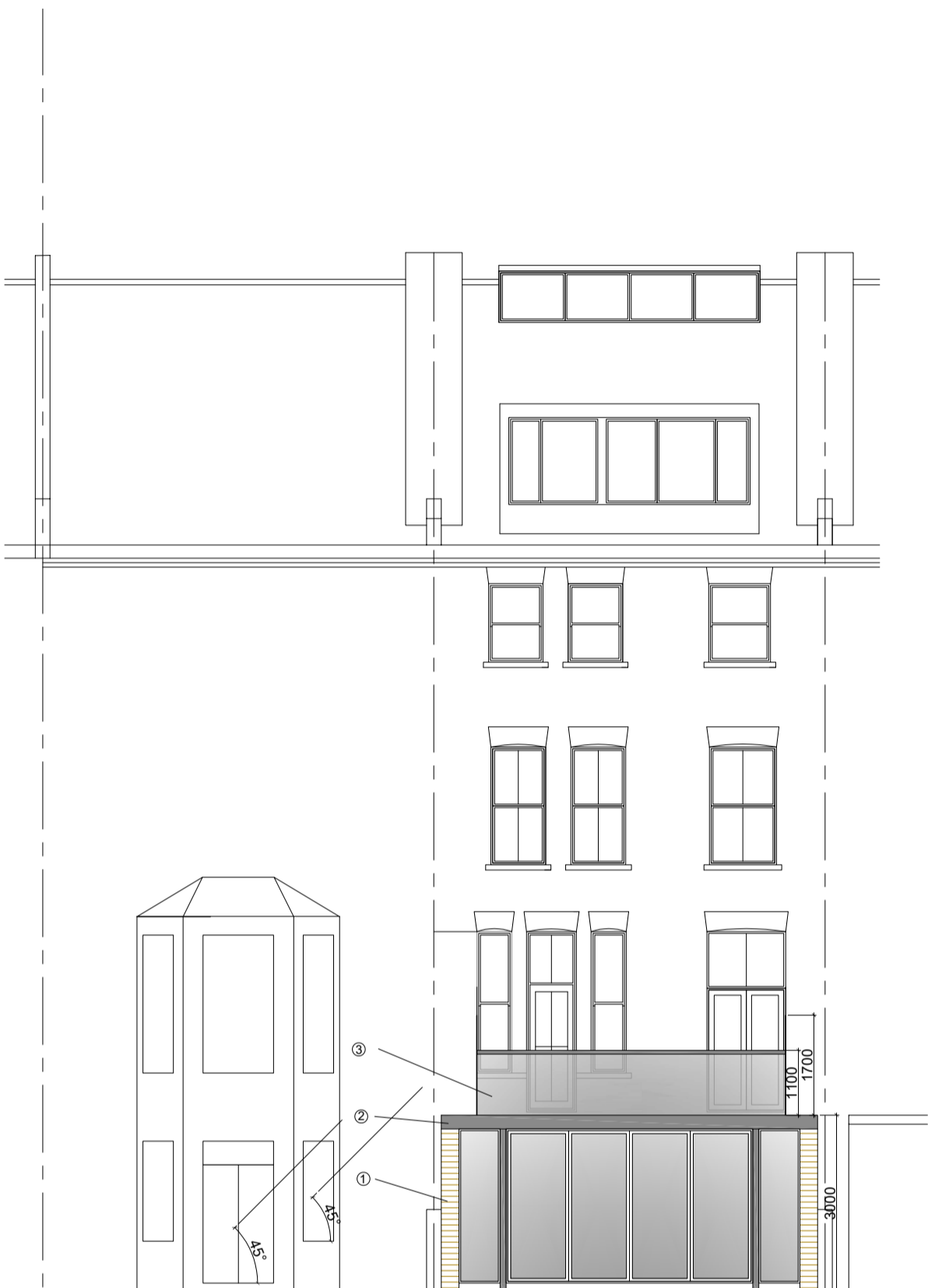
REAR ELEVATION no 14
