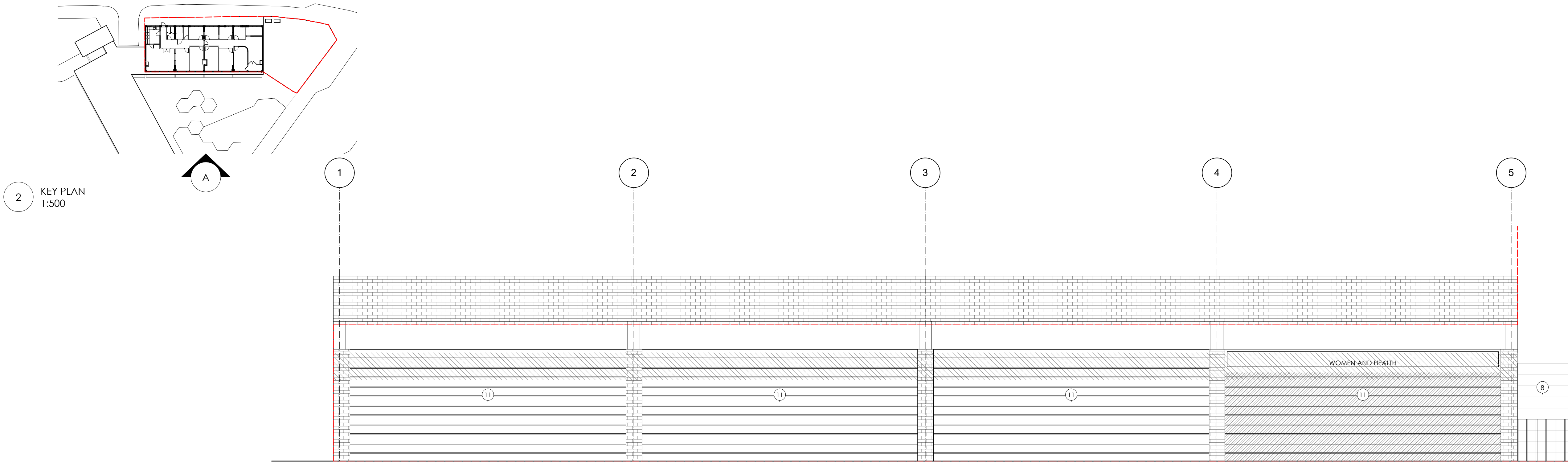
1 PROPOSED - ELEVATION A W/ ROLLER SHUTTERS 1:50
