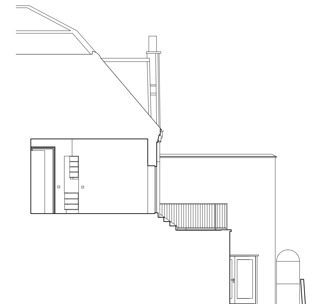
SECTION B-B AS EXISTING
