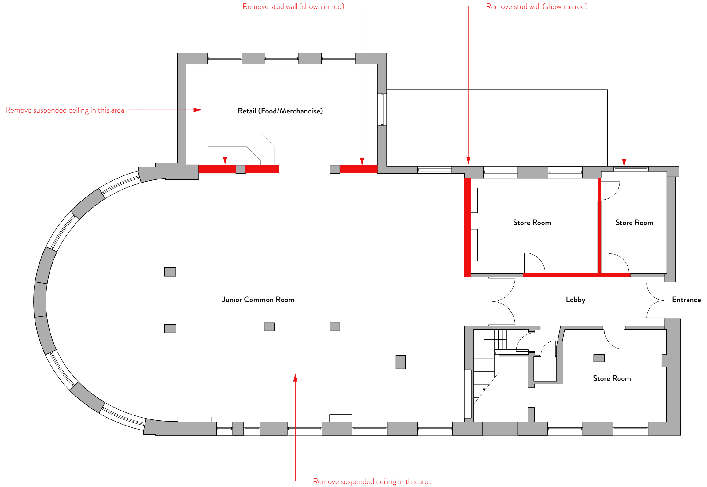
Demolition Plan 1:100
