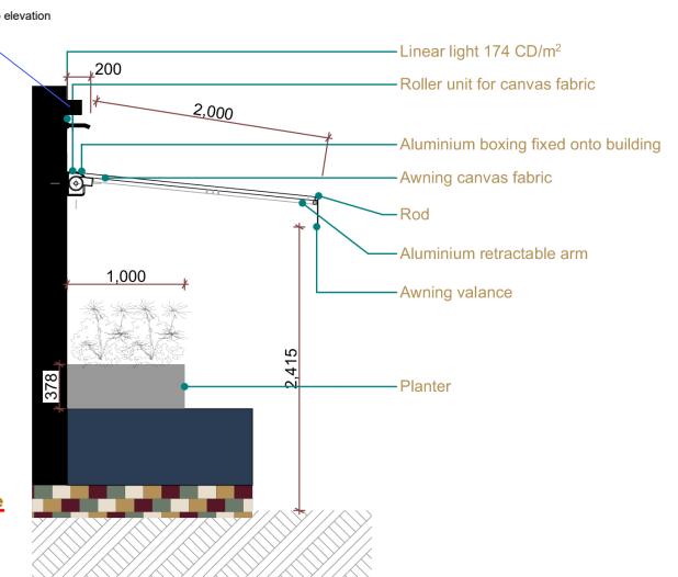
AWNING/PLANTER SECTION
