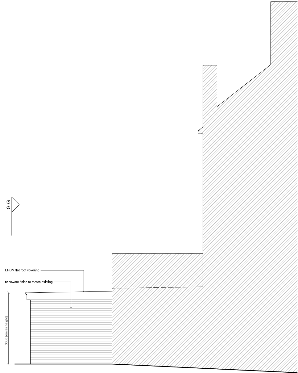
1. PROPOSED SIDE ELEVATION F-F
