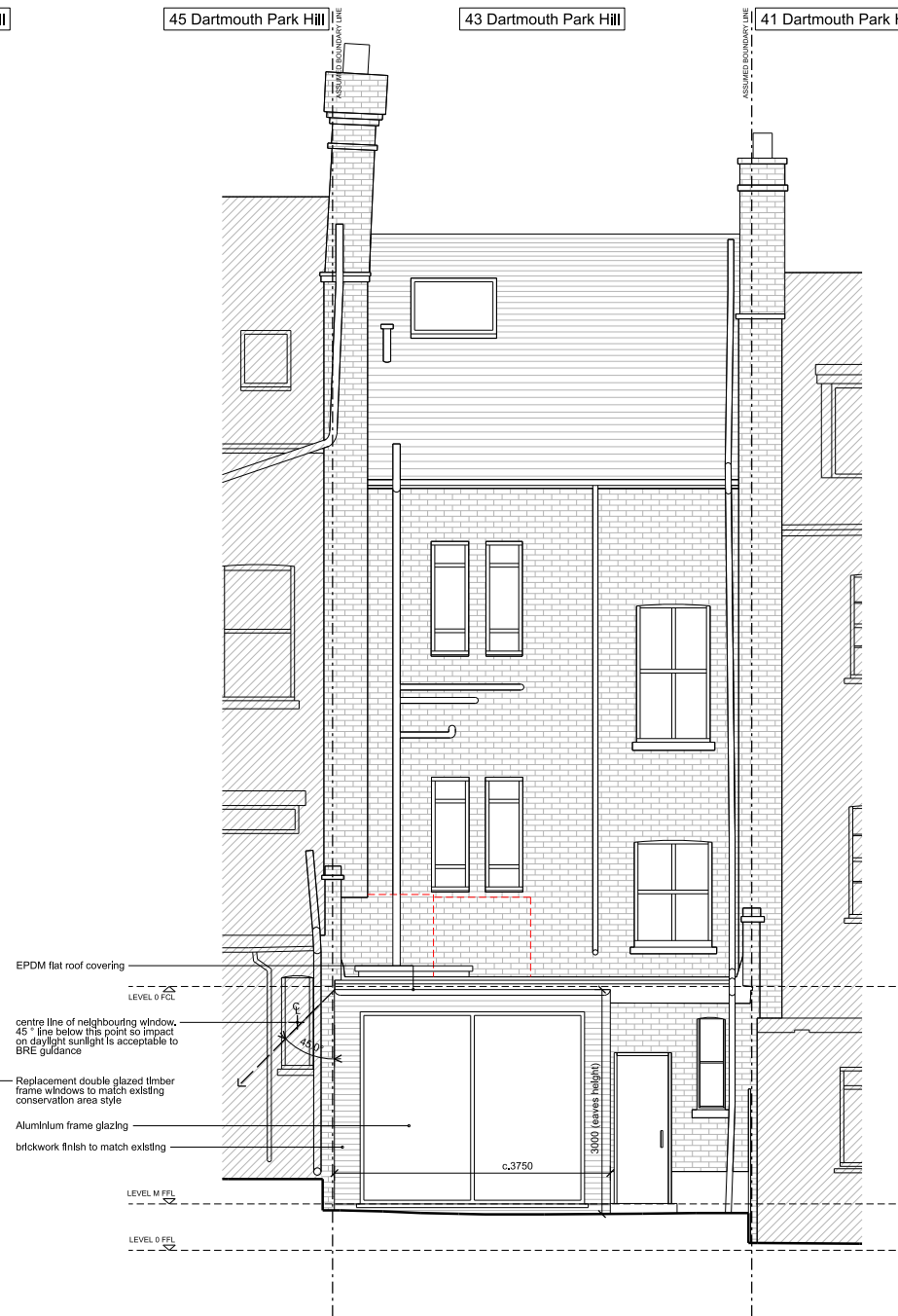
2. PROPOSED REAR ELEVATION G-G
