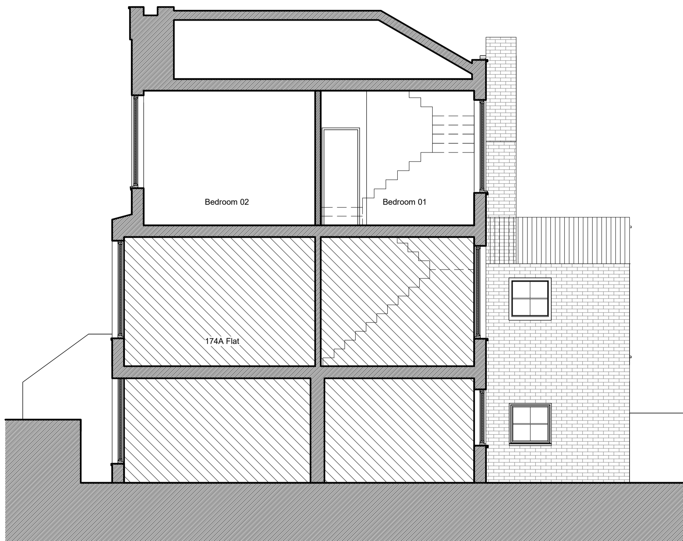
1 Existing Section AA 1:50
