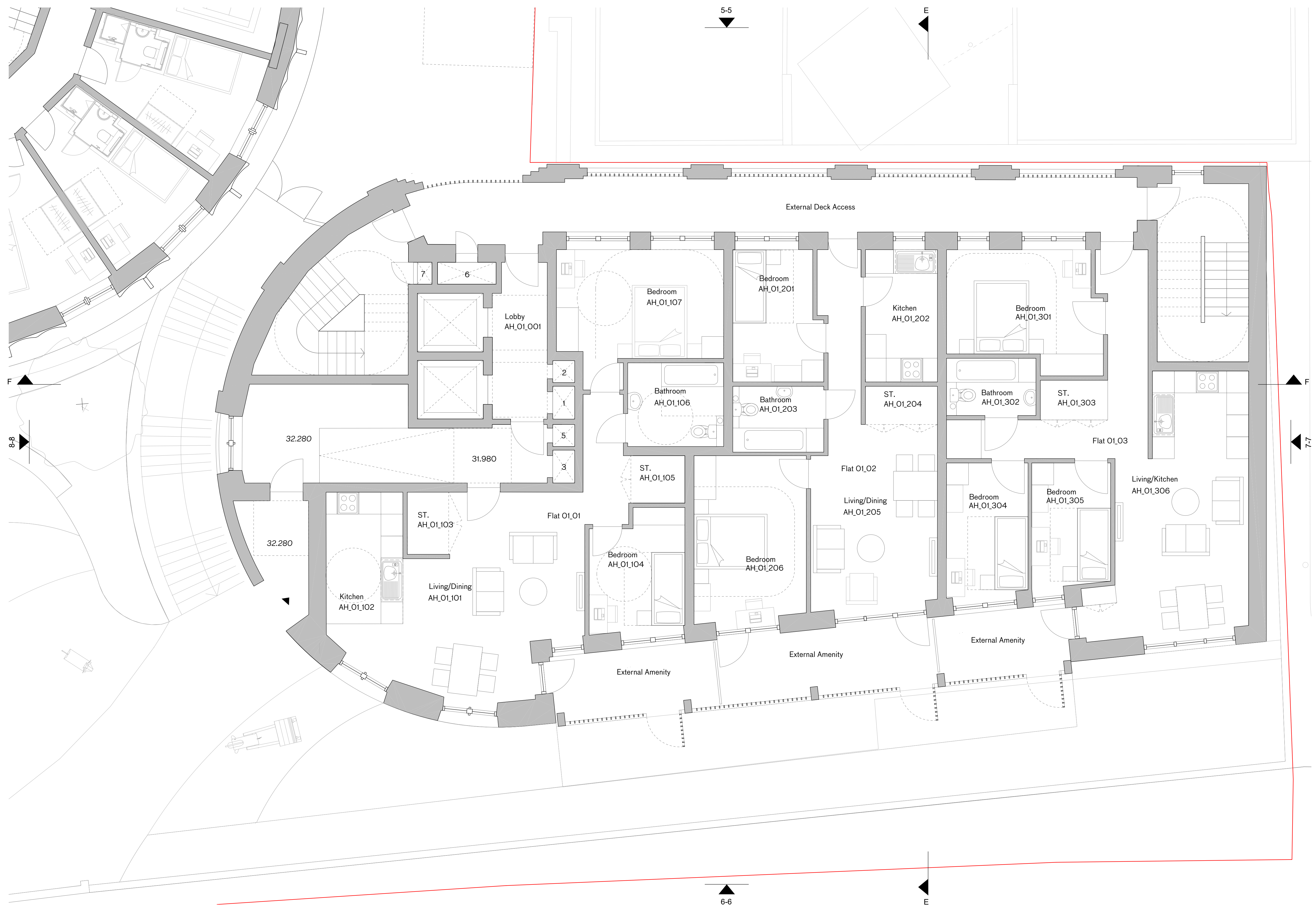
Affordable Housing Level 1 Floor Plan
