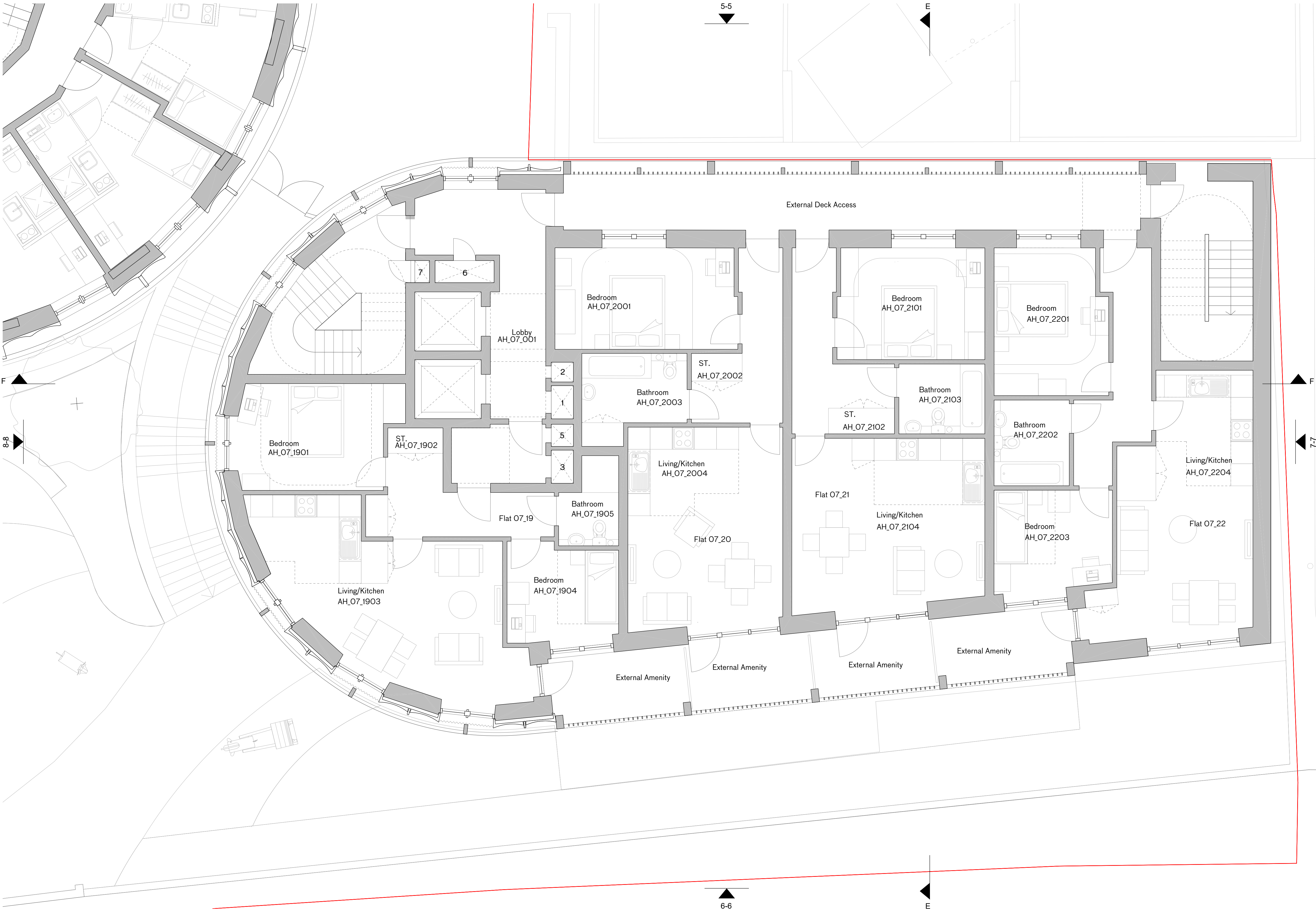
Affordable Housing Level 7 - 8 Floor Plan
