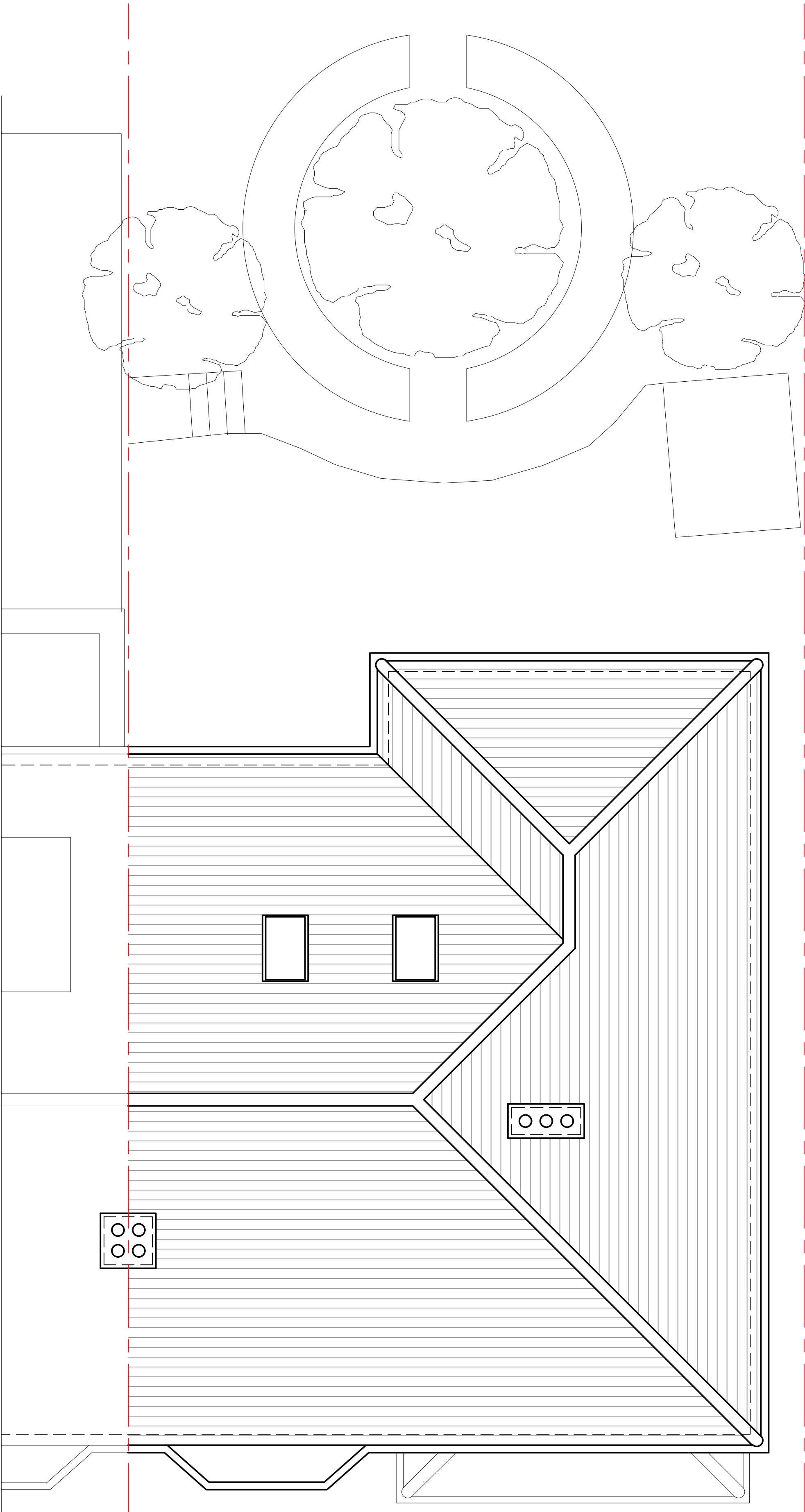
ROOF PLAN - EXISTING scale 1:50
