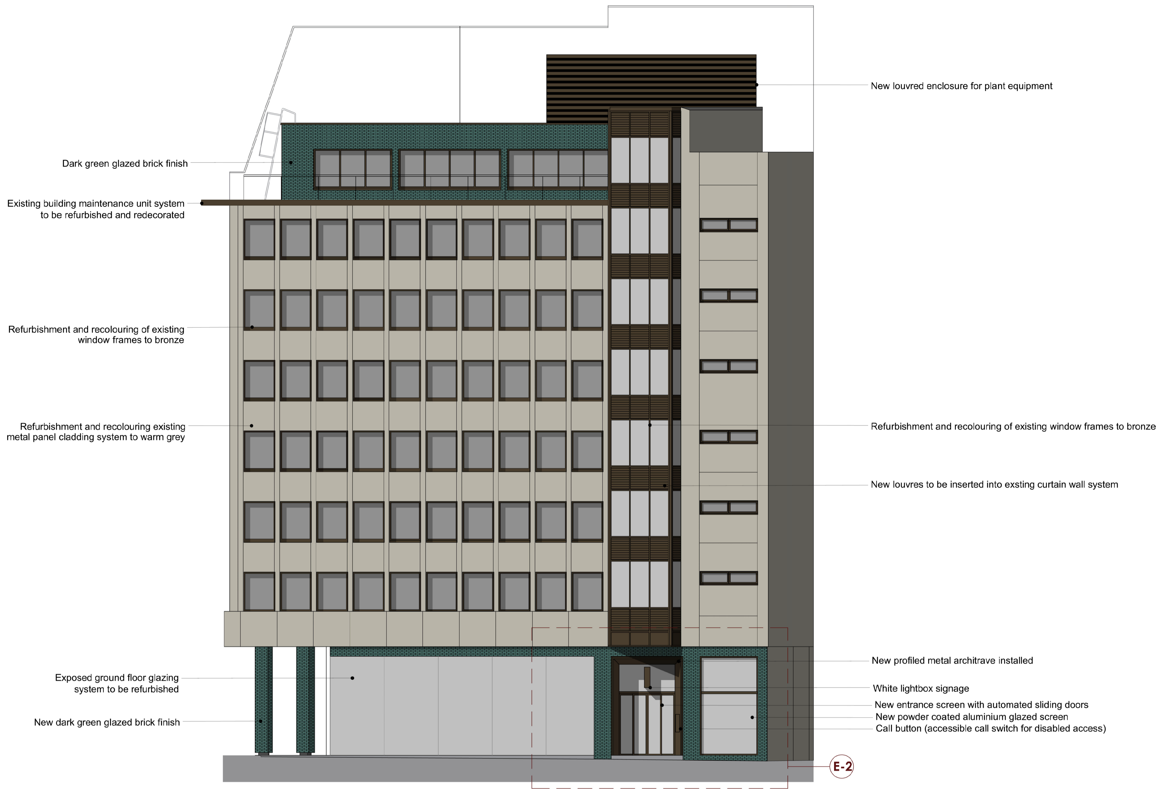
1 Proposed Dyott Street Elevation 1 : 100
