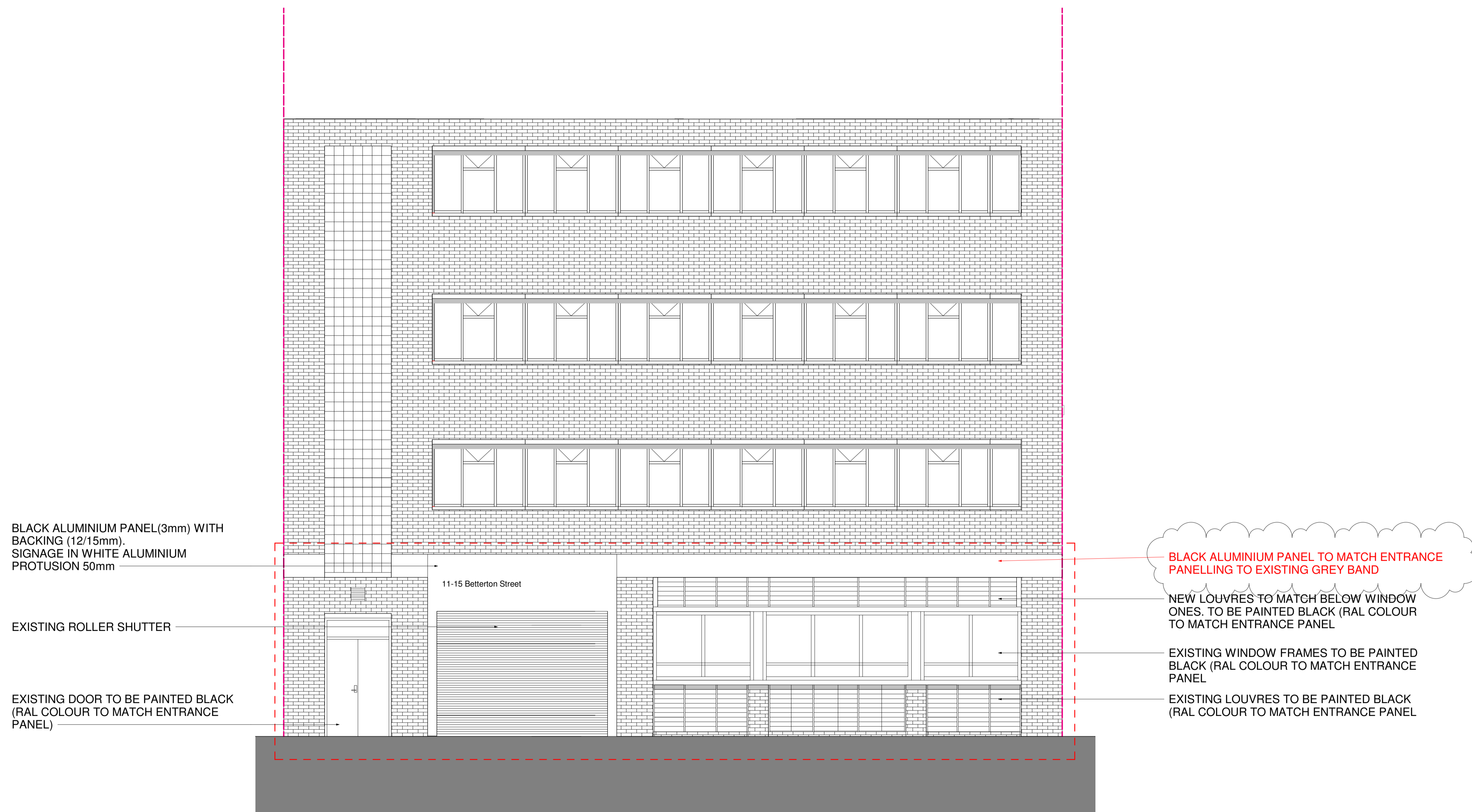
1 Betterton Street Proposed Elevation 2 (ROLLER SHUTTER CLOSED) Scale 1 : 50
