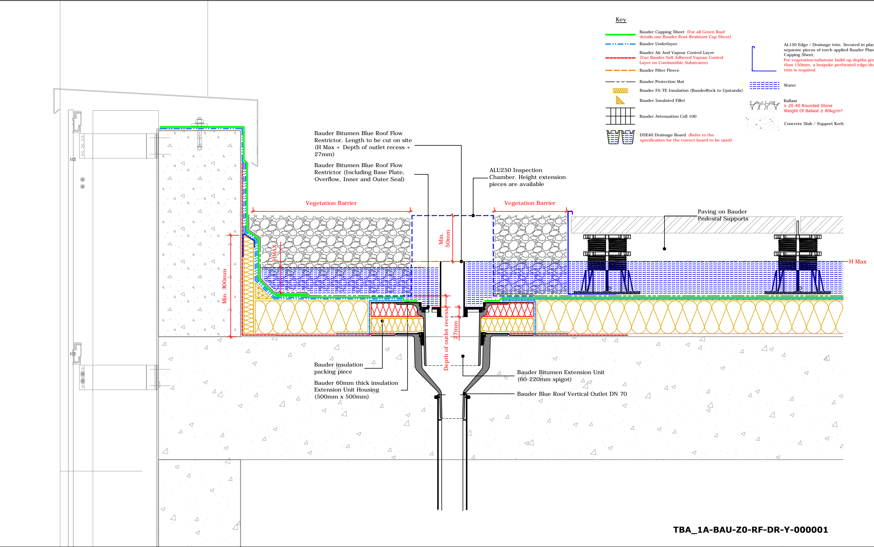
Bespoke Detail 420 & 421
