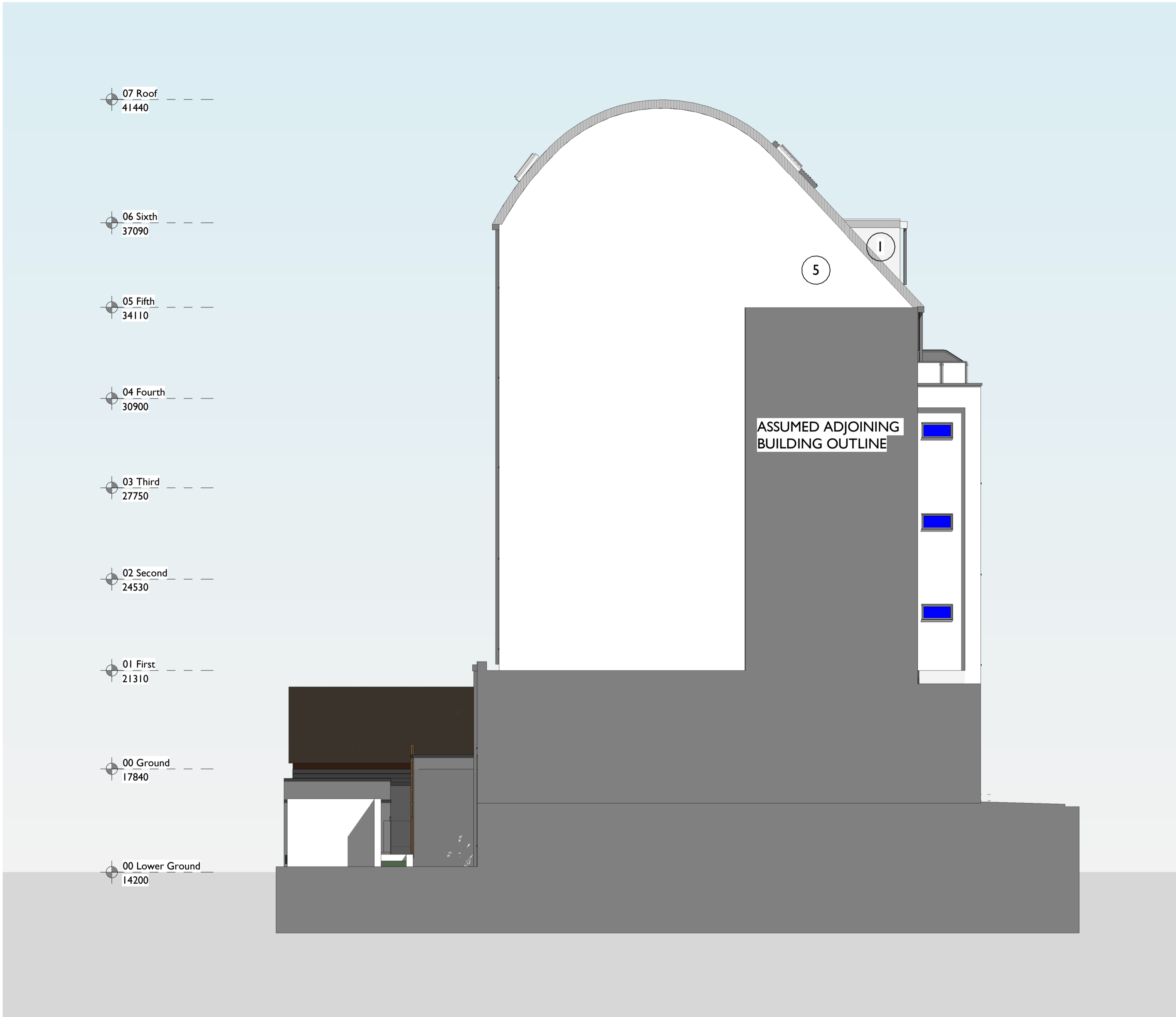
SOUTH ELEVATION 1 : 100
