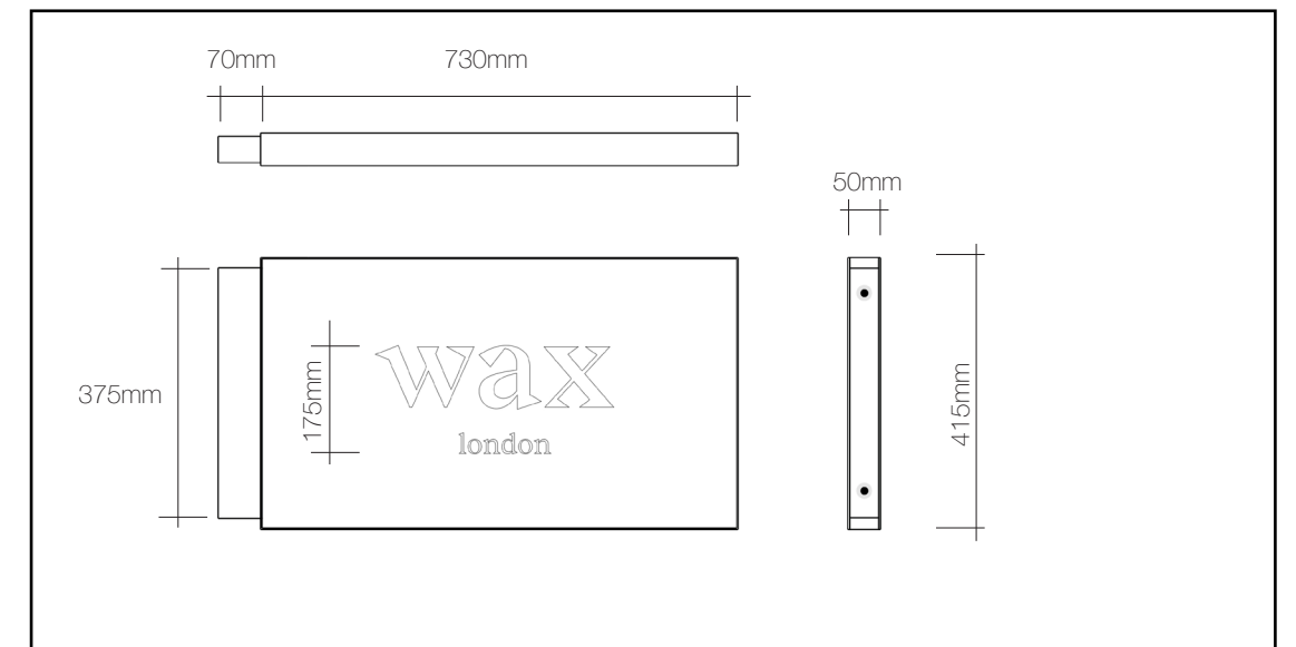
PROJECTING SIGN DETAIL
