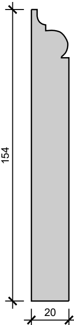
Skirting Type B
