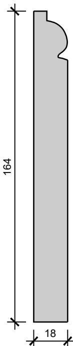
Skirting Type C
