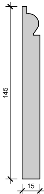
Skirting Type A
