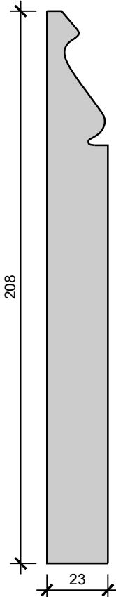
Skirting Type E
