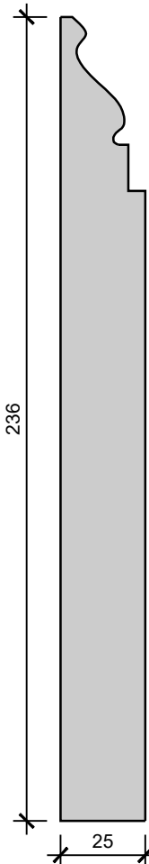
Skirting Type G
