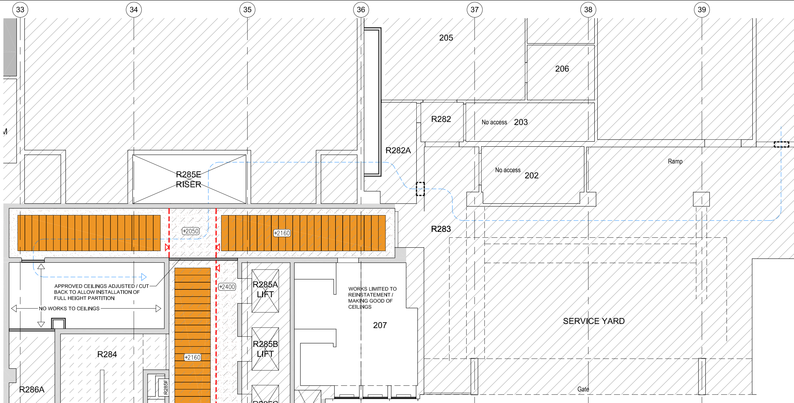
1 LEVEL 2 - CORE A - REFLECTED CEILING PLAN AS PROPOSED 1:50
