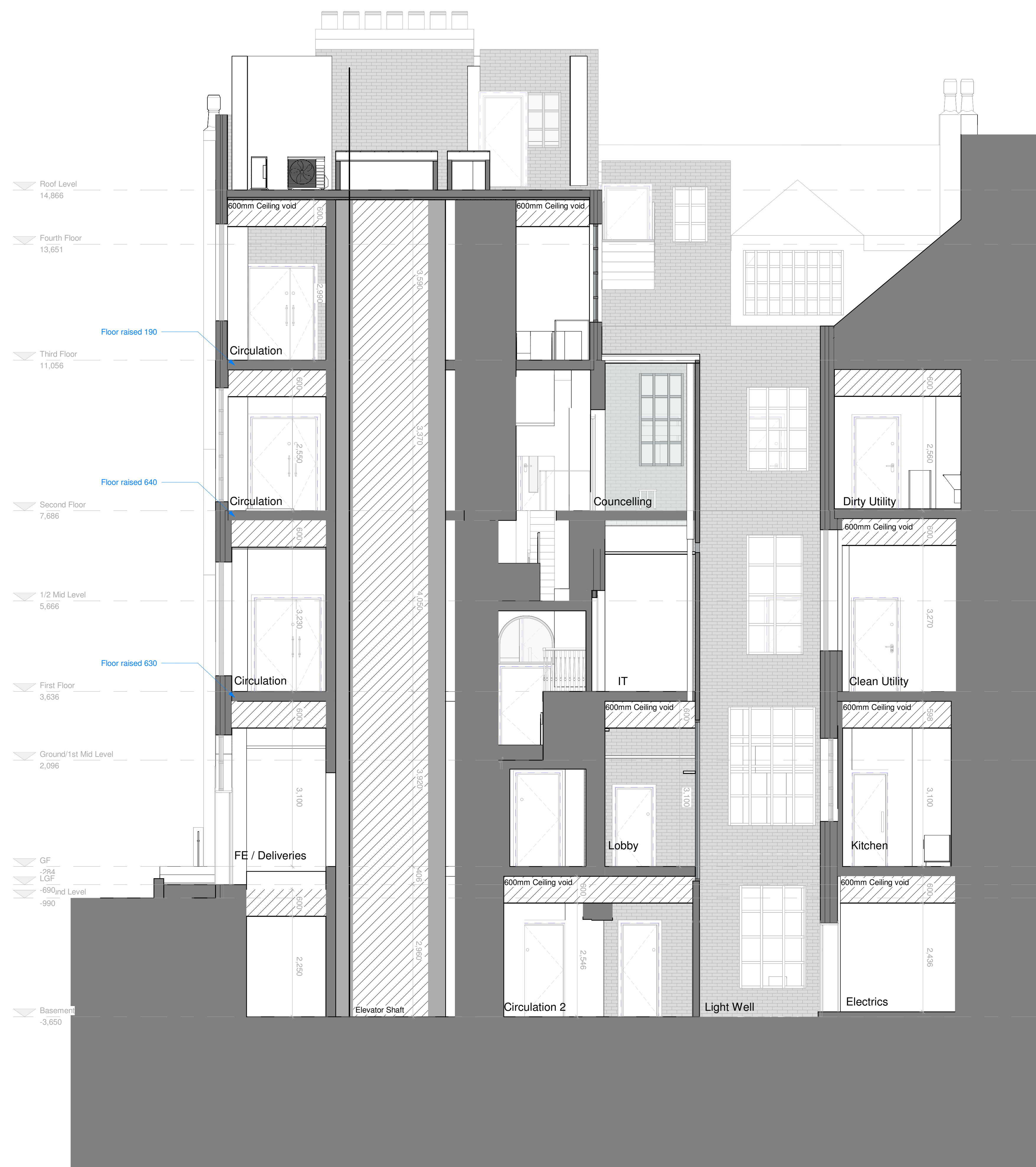
Proposed Section C - C 1 : 50
