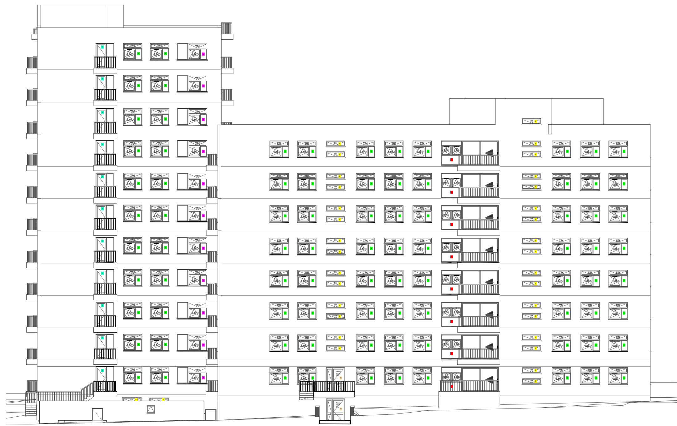
1 Sheringham North East Proposed Elevation 1 : 200
