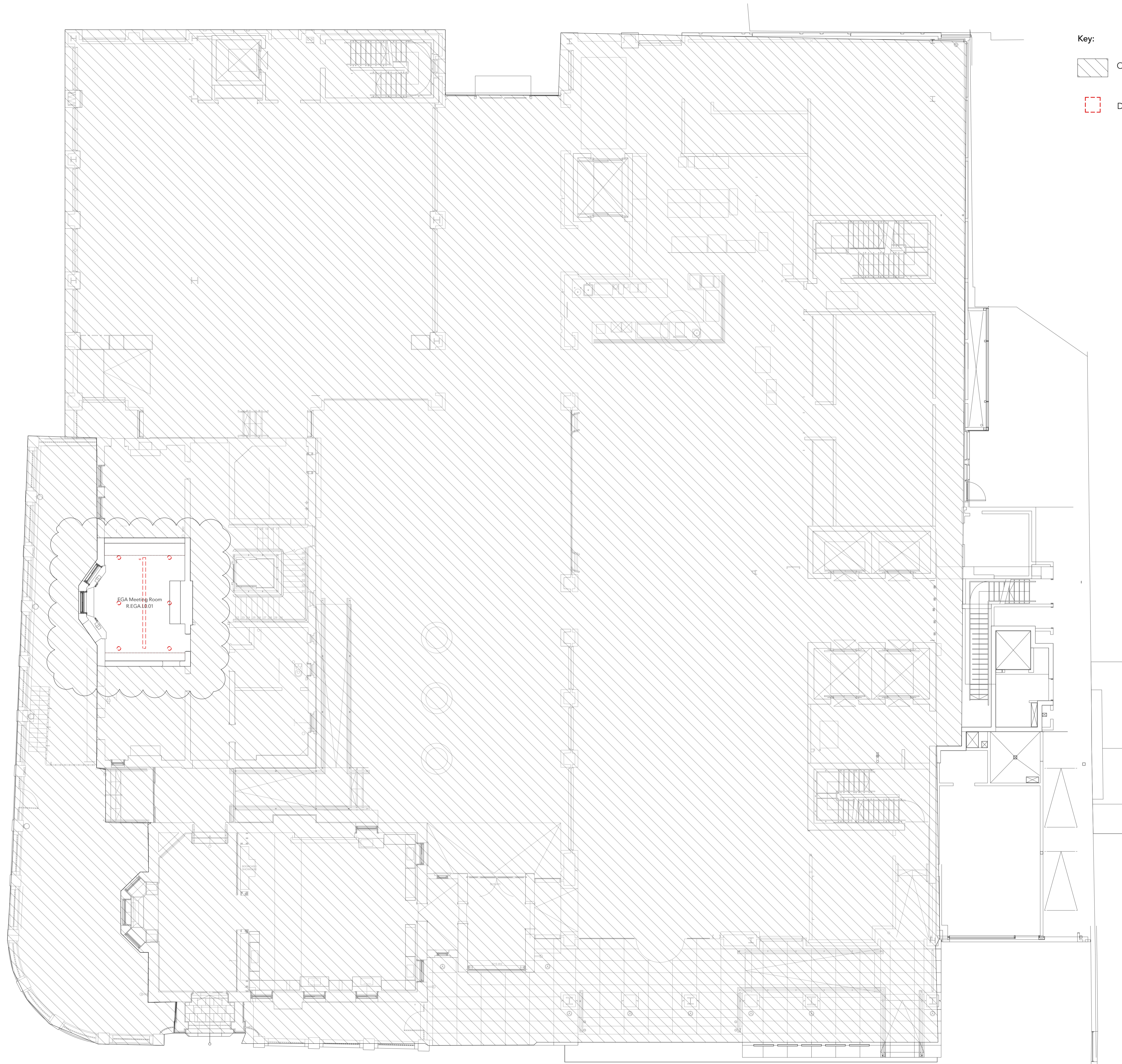
1 Ground Floor Demolition Ceiling Scale: 1:100
