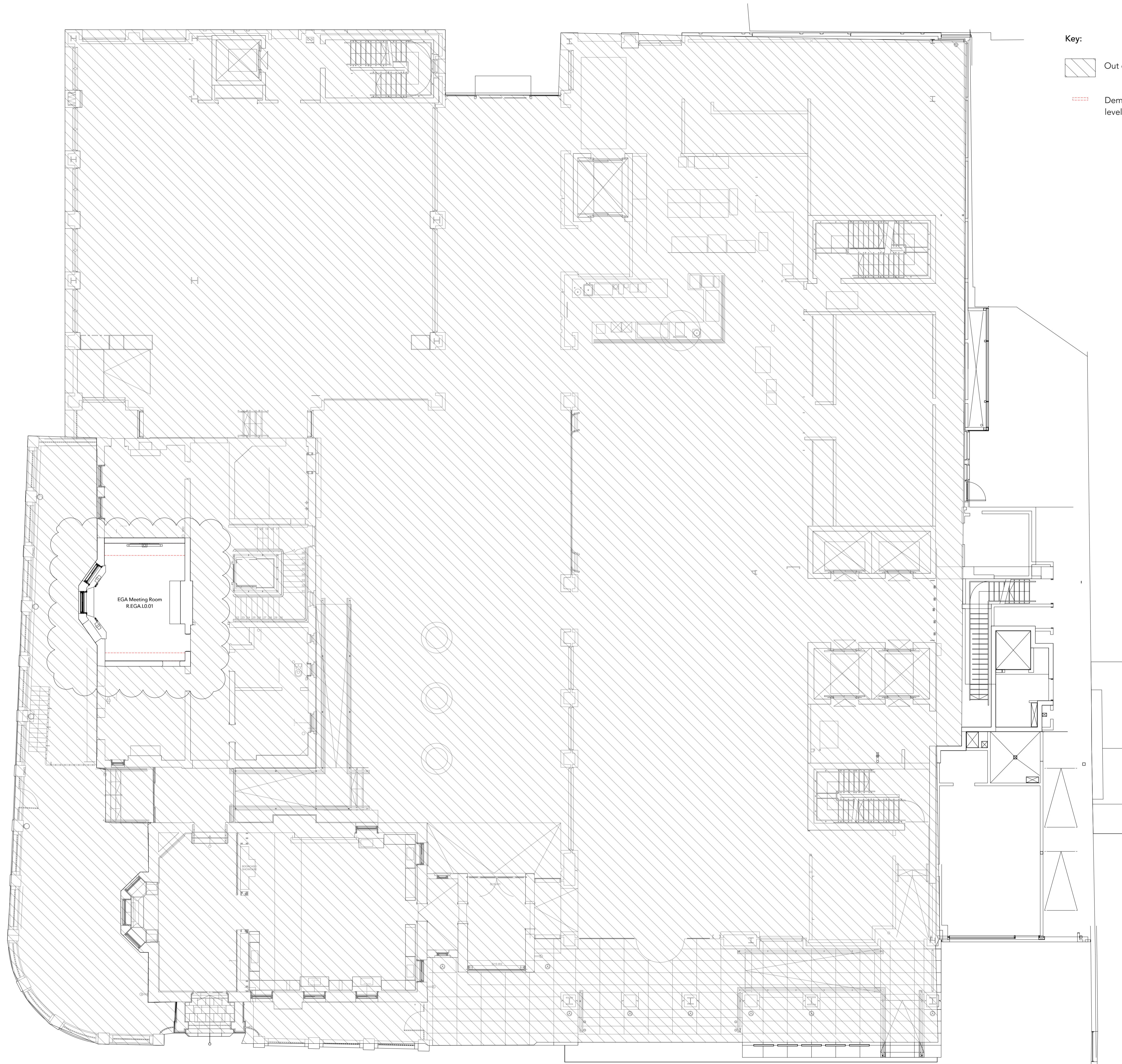
1 Ground Floor Demolition Scale: 1:100
