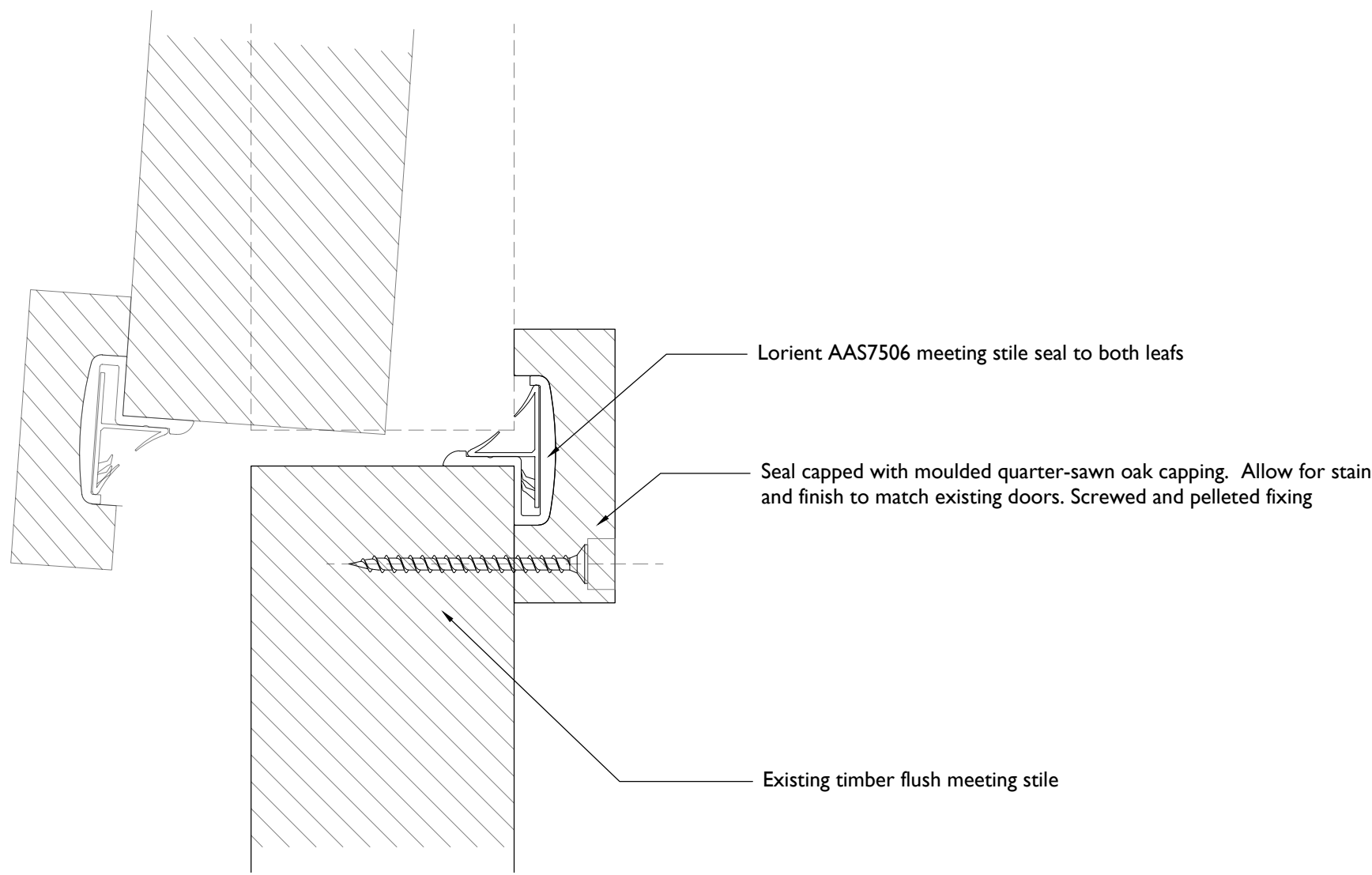
4 MEETING STILE DETAIL 1:1
