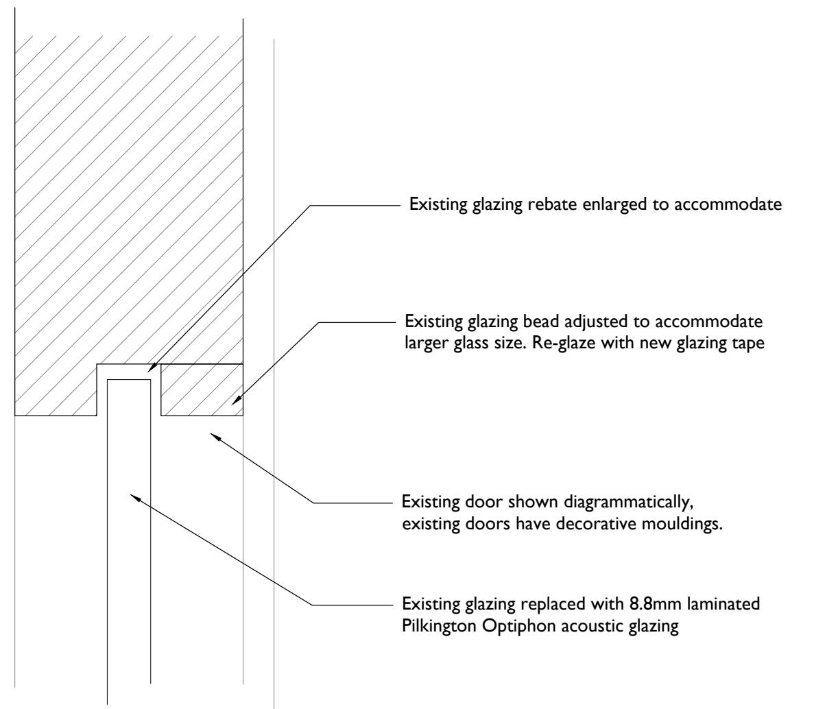
3 DOOR GLAZING DETAIL 1:1
