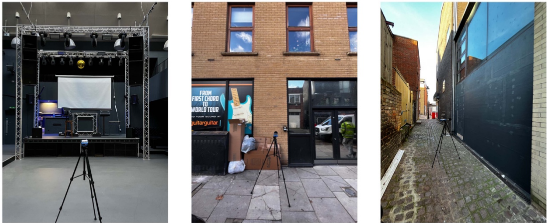
Figure 2 – Measurement Locations
