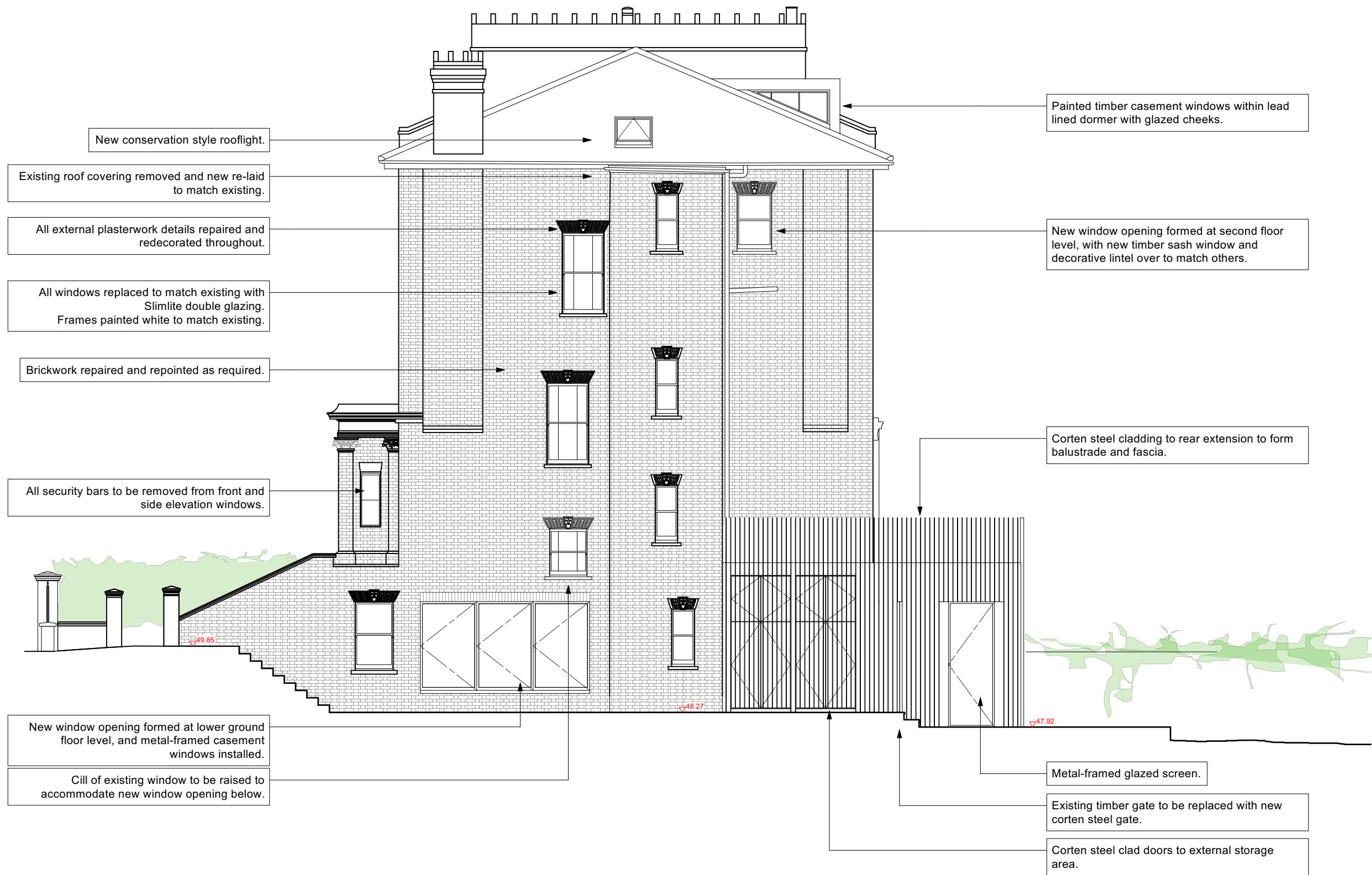
1 Proposed Side (South-West) Elevation Scale: 1:100
