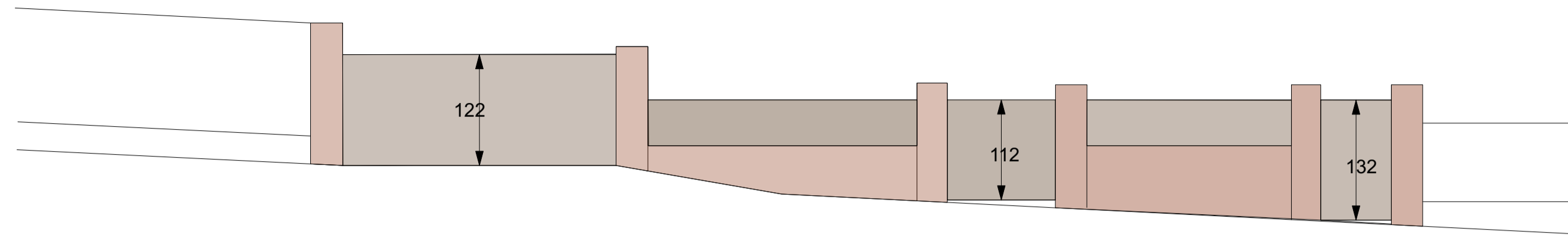
front boundary - materials as already approved in drawing CD_018_A position of gates to fit this design adjusted as shown above
