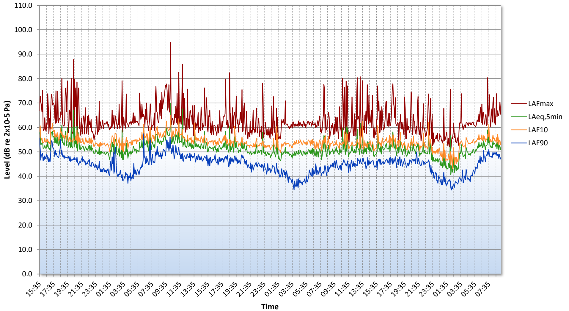
Figure 28138.TH1
