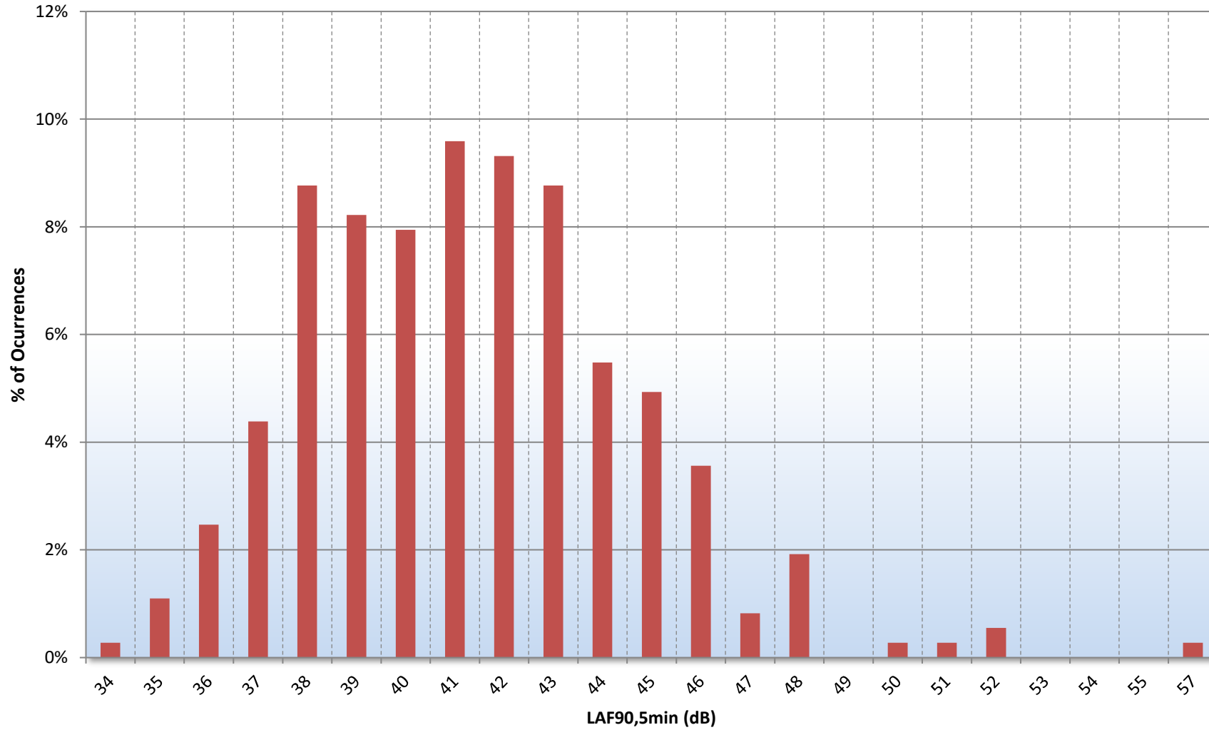
Figure 28138.Night-time L90.TH1
