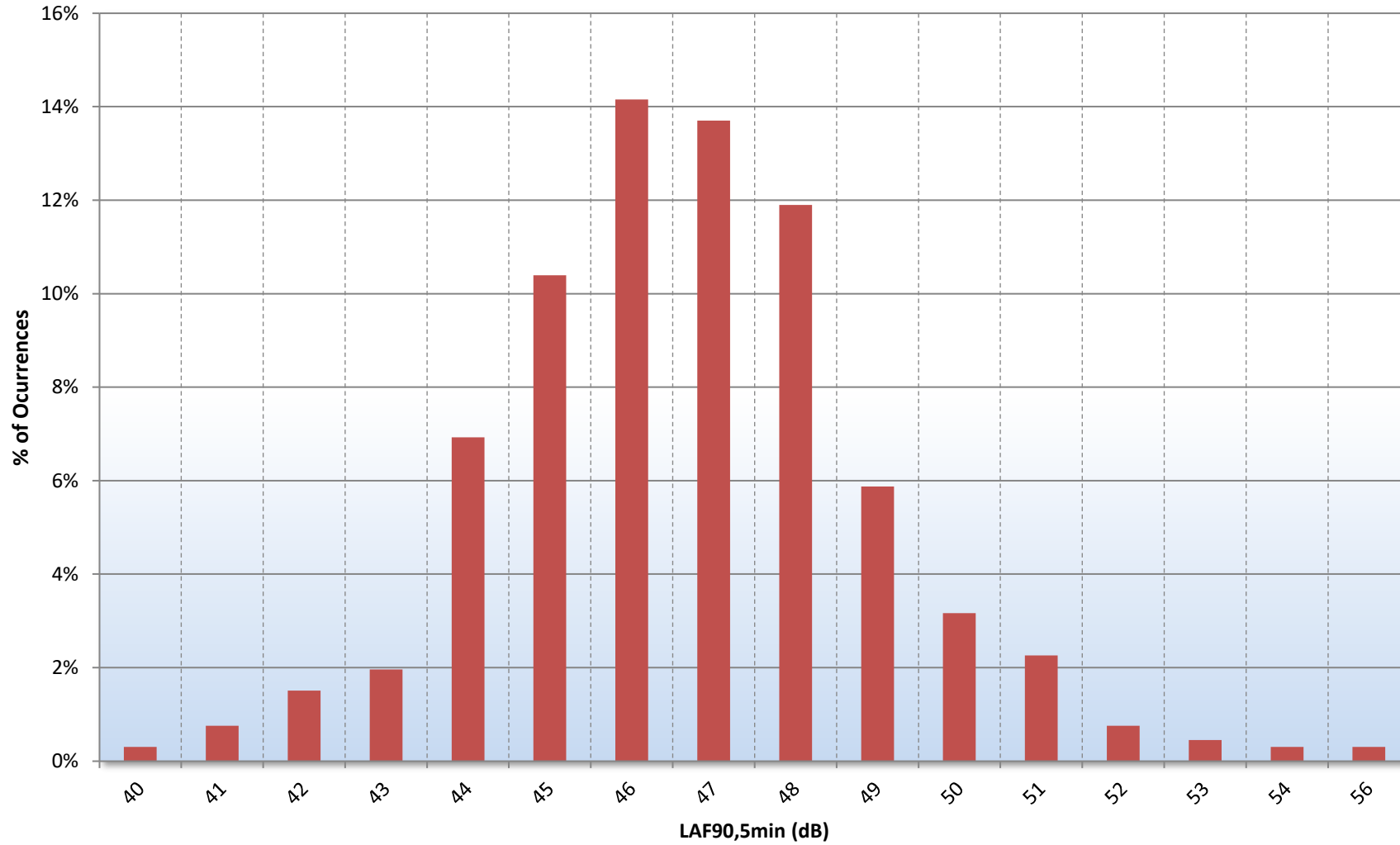
Figure 28138.Daytime L90.TH1
