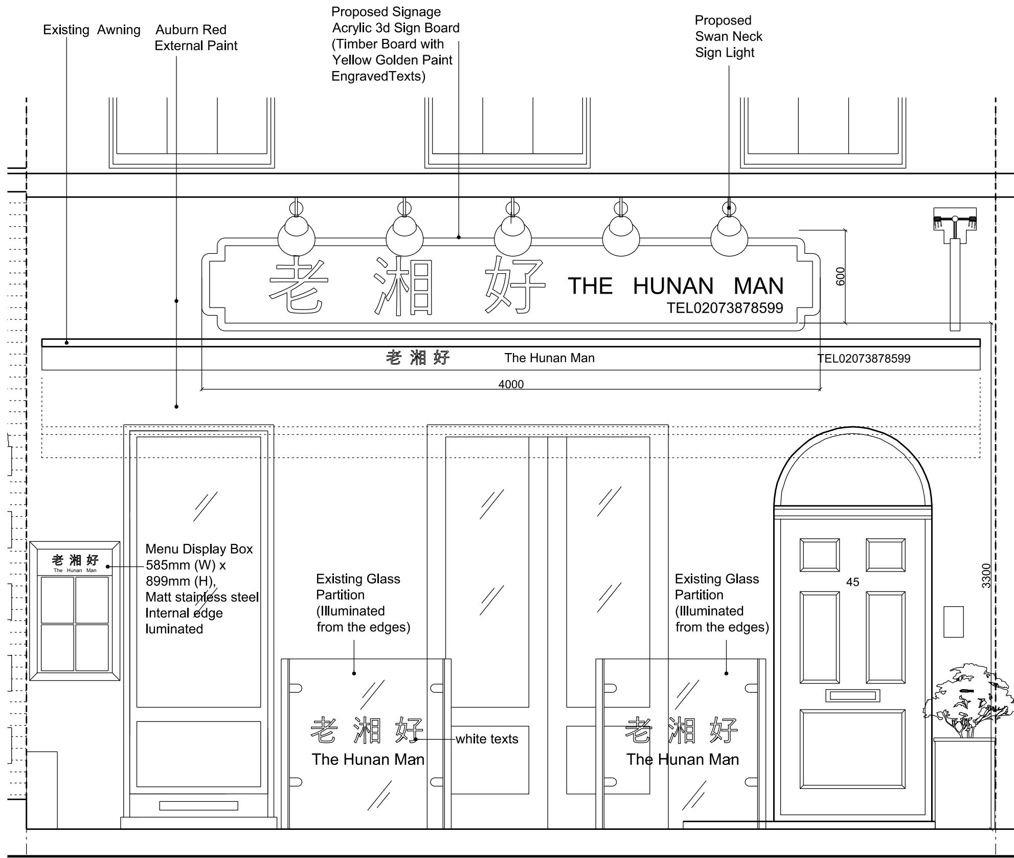
01 PROPOSED SHOPFRONT AND ADVERTISEMENT A-E-01 Scale 1:25
