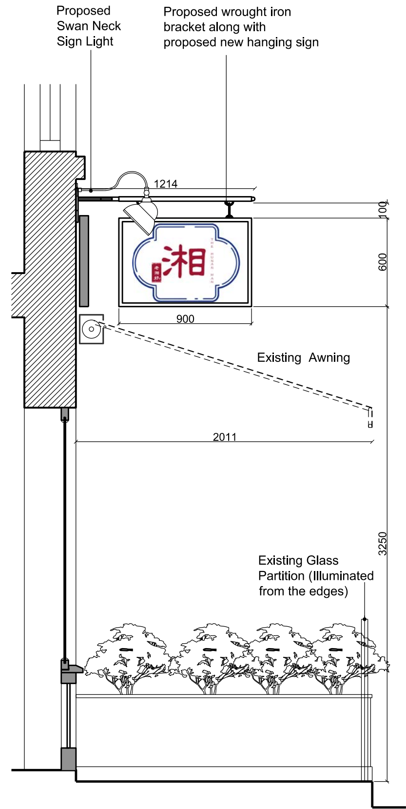
02 SECTION - PROPOSED SHOPFRONT A-E-01 Scale 1:25
