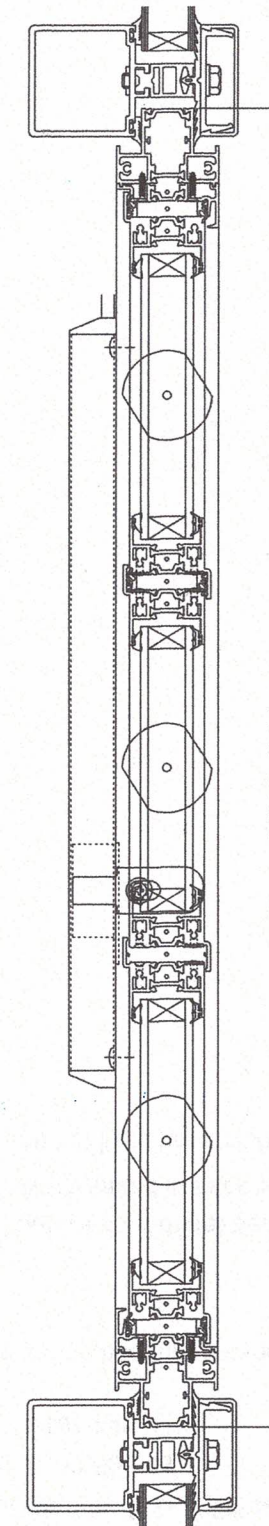
28mm glazing channel 24V dc D&H actuator
