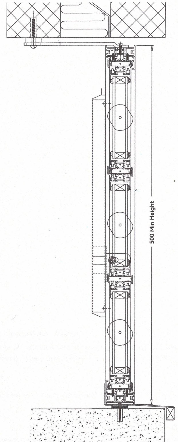
Equal frame & pressed cill 24V dc D&H actuator
