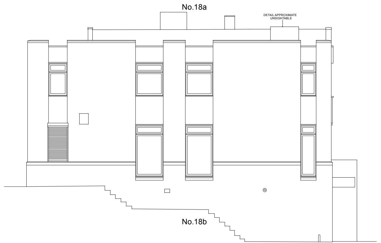
DATUM 106.00m A.O.D. No.18a FROGNAL GARDENS SIDE/WEST ELEVATION
