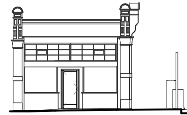
EXISTING SOUTH END ROAD ELEVATION
