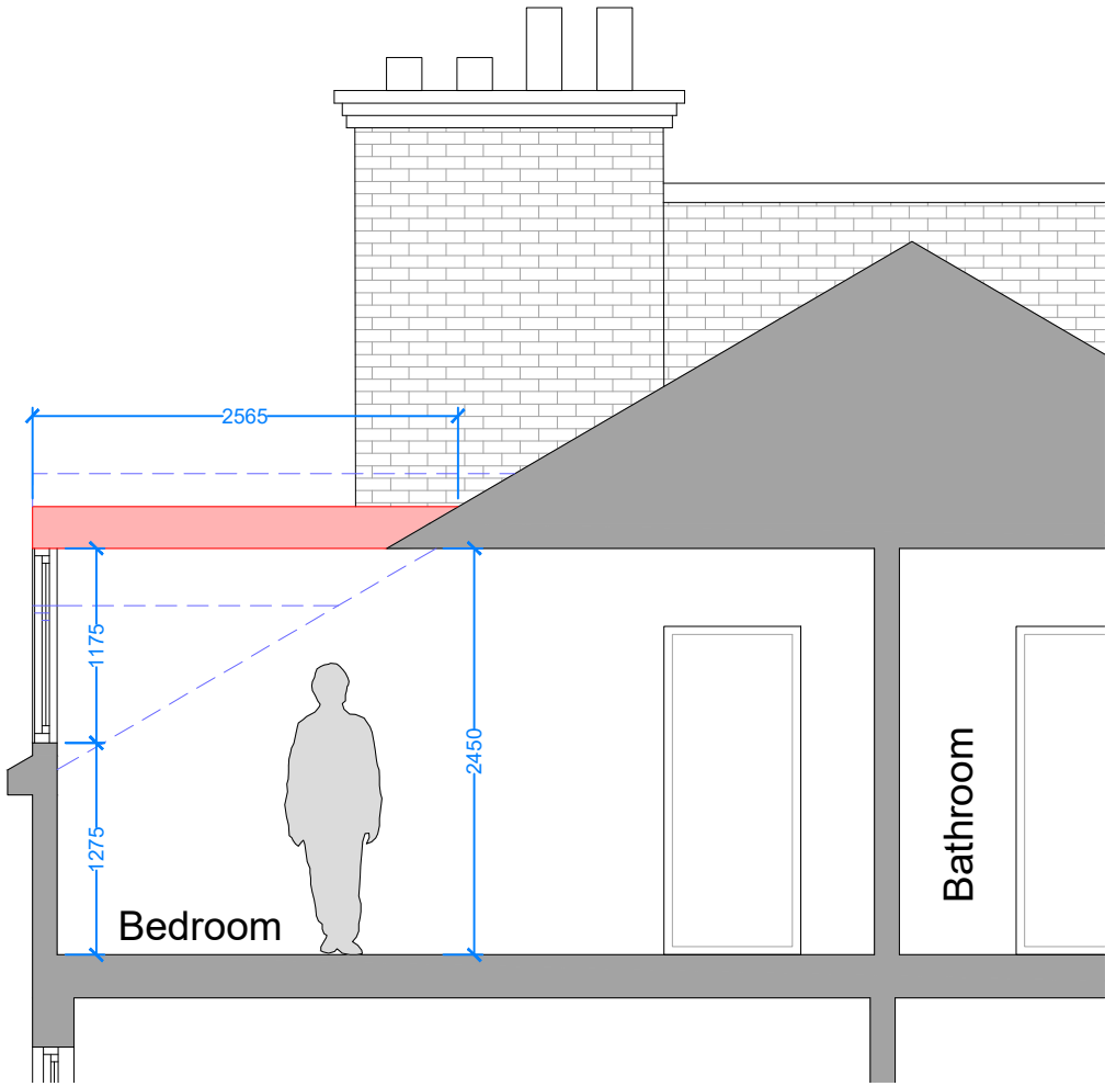
02 Proposed Section 1:50 @ A3
