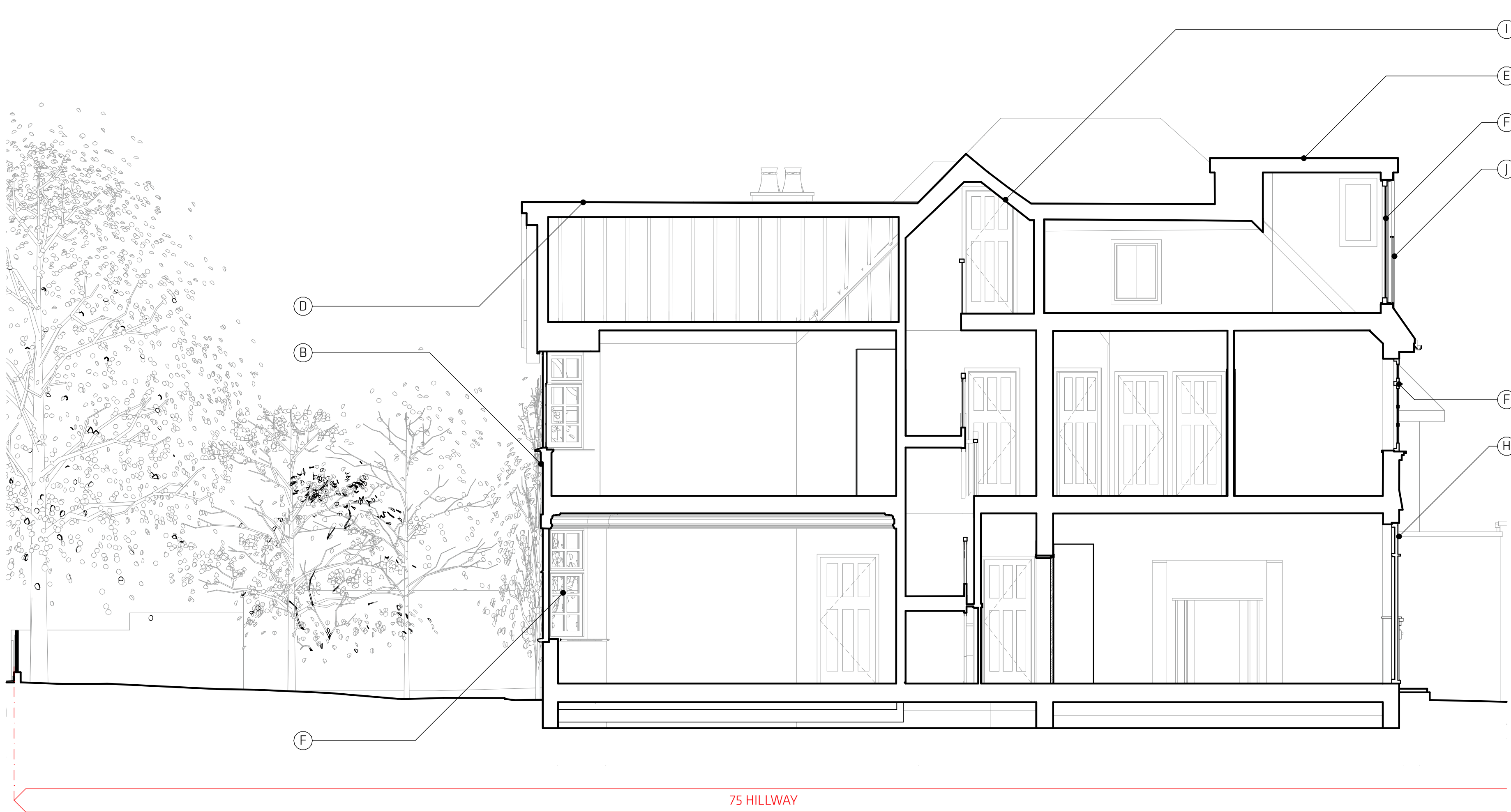
02 Existing Section BB Scale @ A1: 1:50
