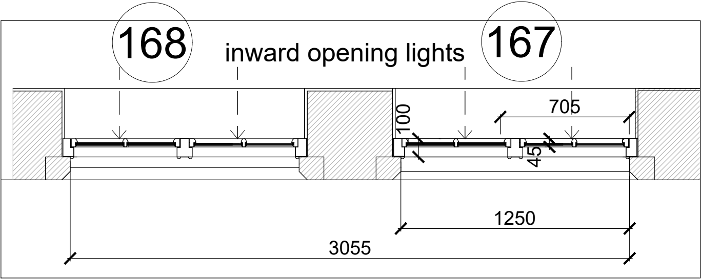
PLAN TYPE 1 PIVOT WINDOW TO KITCHEN
