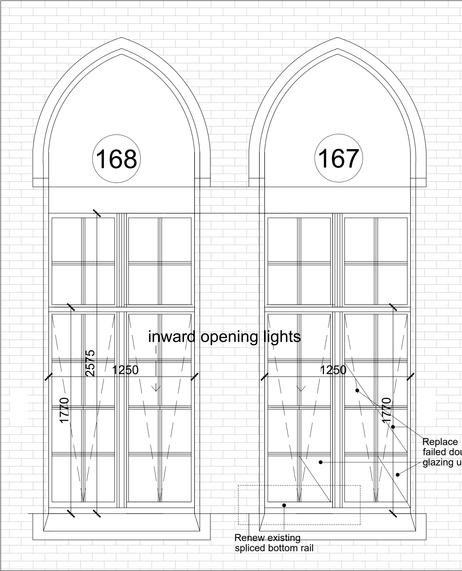
ELEVATION TYPE 1 PIVOT WINDOW
